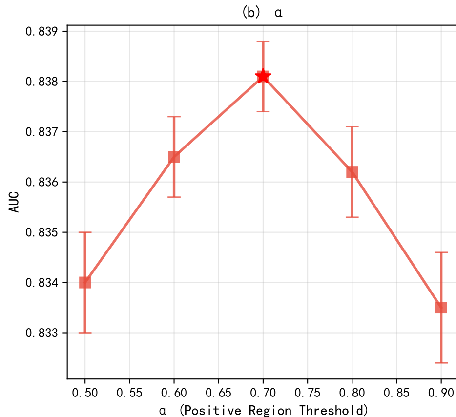
Figure 4-5: Hyperparameter Sensitivity Analysis
