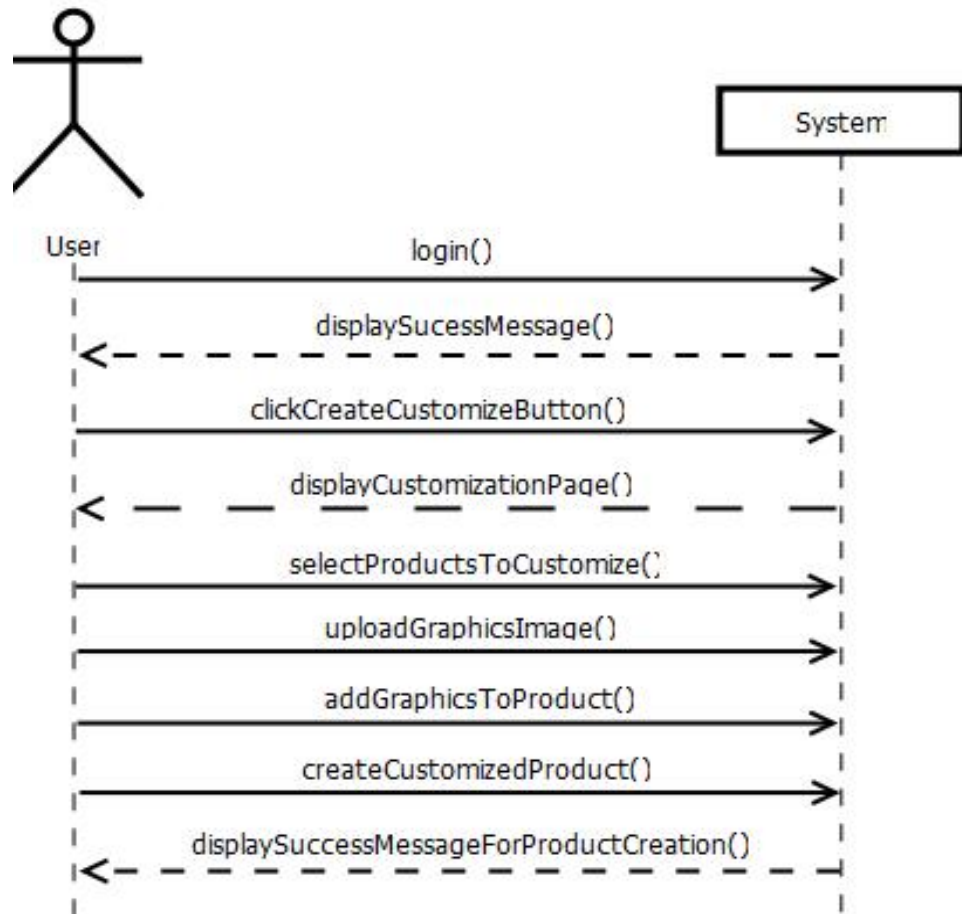
Figure 3.4.2.2: System Sequence Diagram for Product Customization
