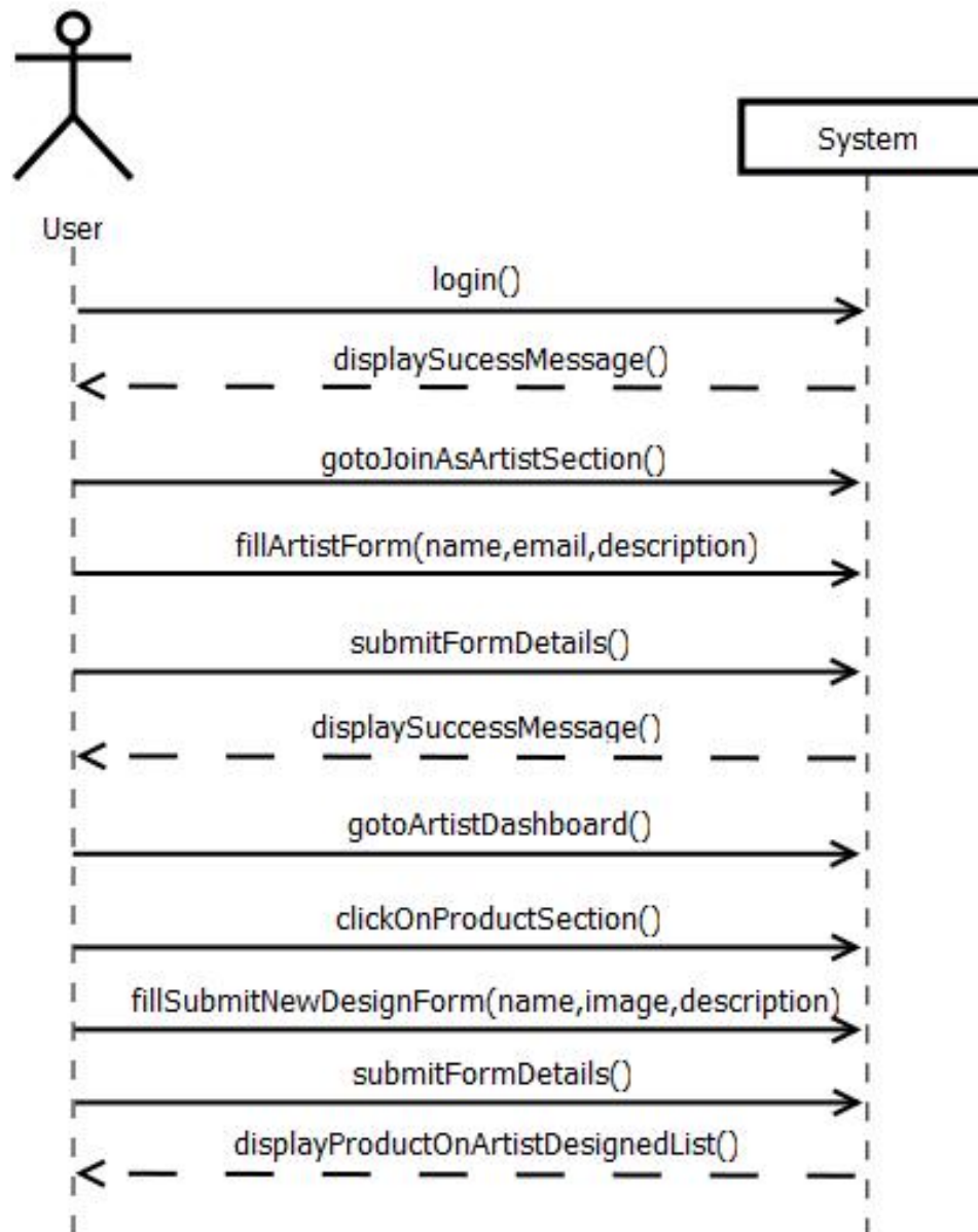
Figure 3.4.2.1: System Sequence Diagram for Artist Design Submission
