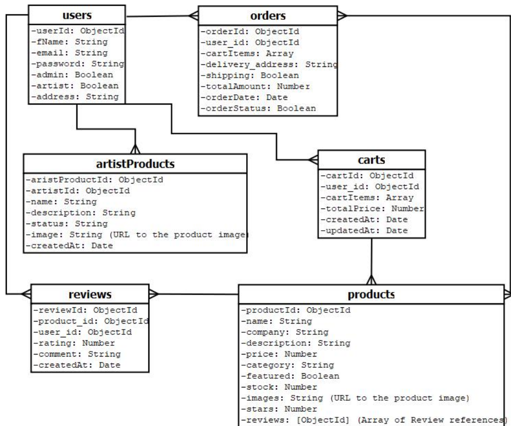
Figure 3.2.1.1: Database Schema of MerchVault
