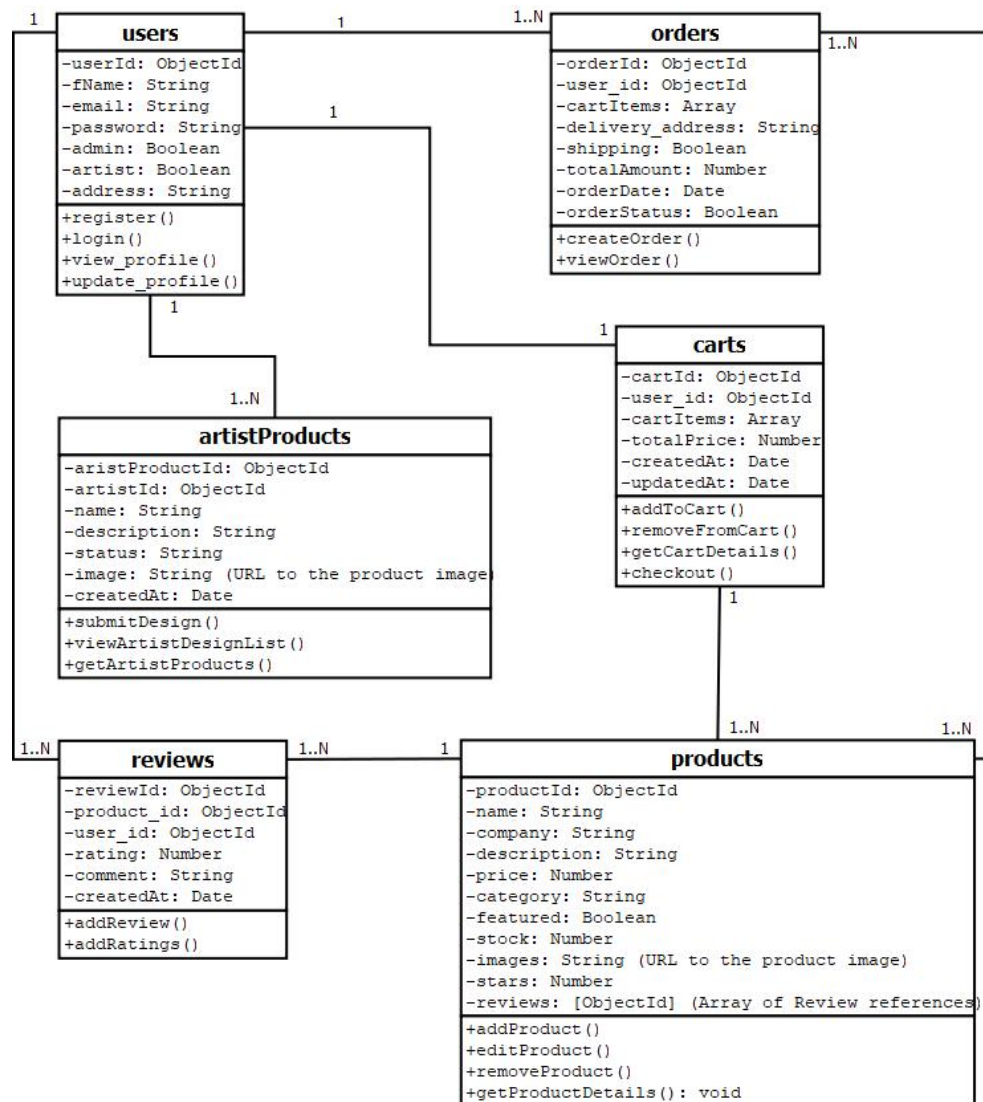
Figure 3.4.3.1: Design Class Diagram of MerchVault
