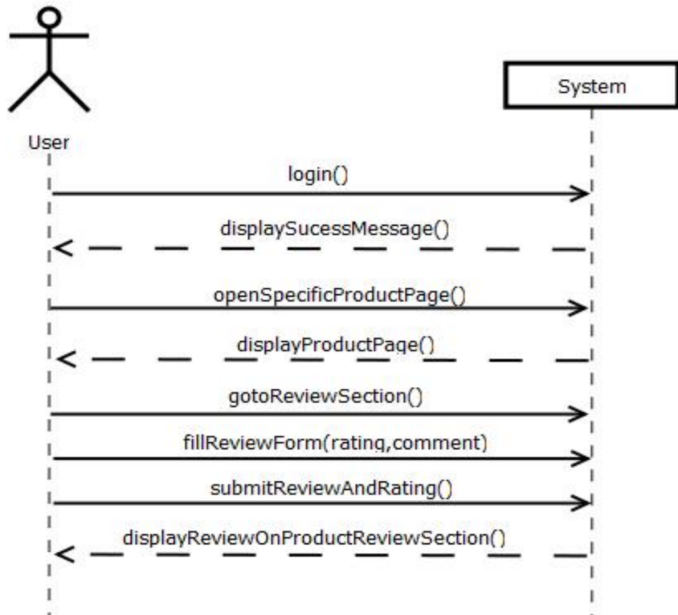
Figure 3.4.2.3: System Sequence Diagram for Product Rating and Reviewing
