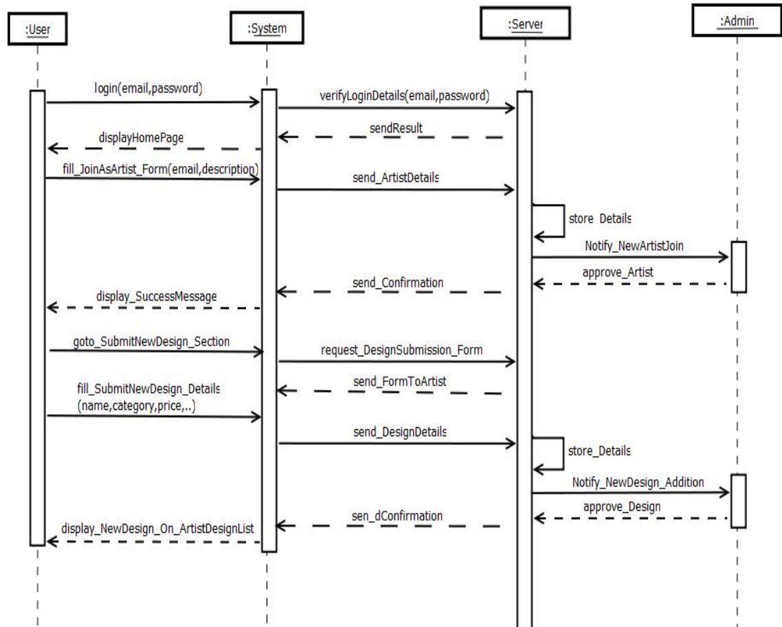
Figure 3.4.4.1: Interaction Diagram for New Design Submission of MerchVault
