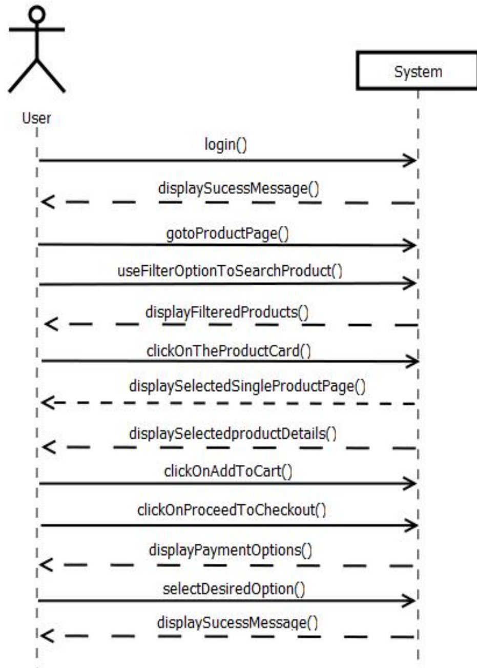
Figure 3.4.2.4: System Sequence Diagram for Product Filtering and Ordering
