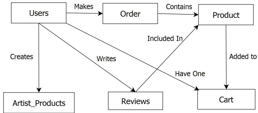
Figure 3.2.1: Block Diagram of Database Collections
