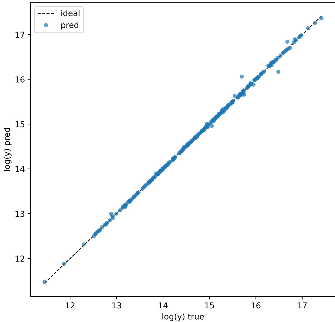
Predictions vs Truth (log space)
