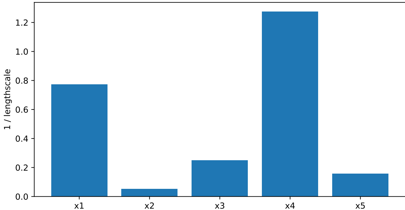
Inverse Lengthscale (Feature Relevance)
