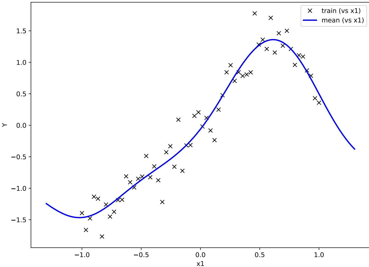
GP (ARD) mean vs x1 (D=3)
