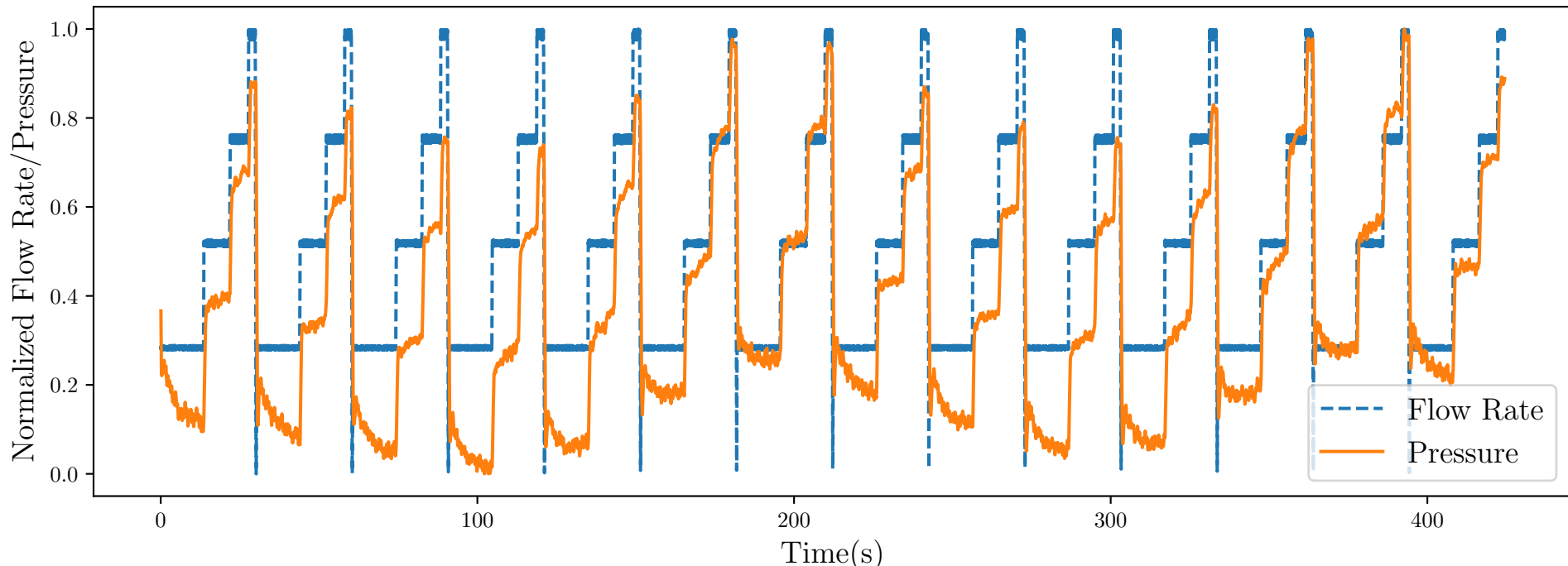
Visualization of pressure changes to set flow rates
