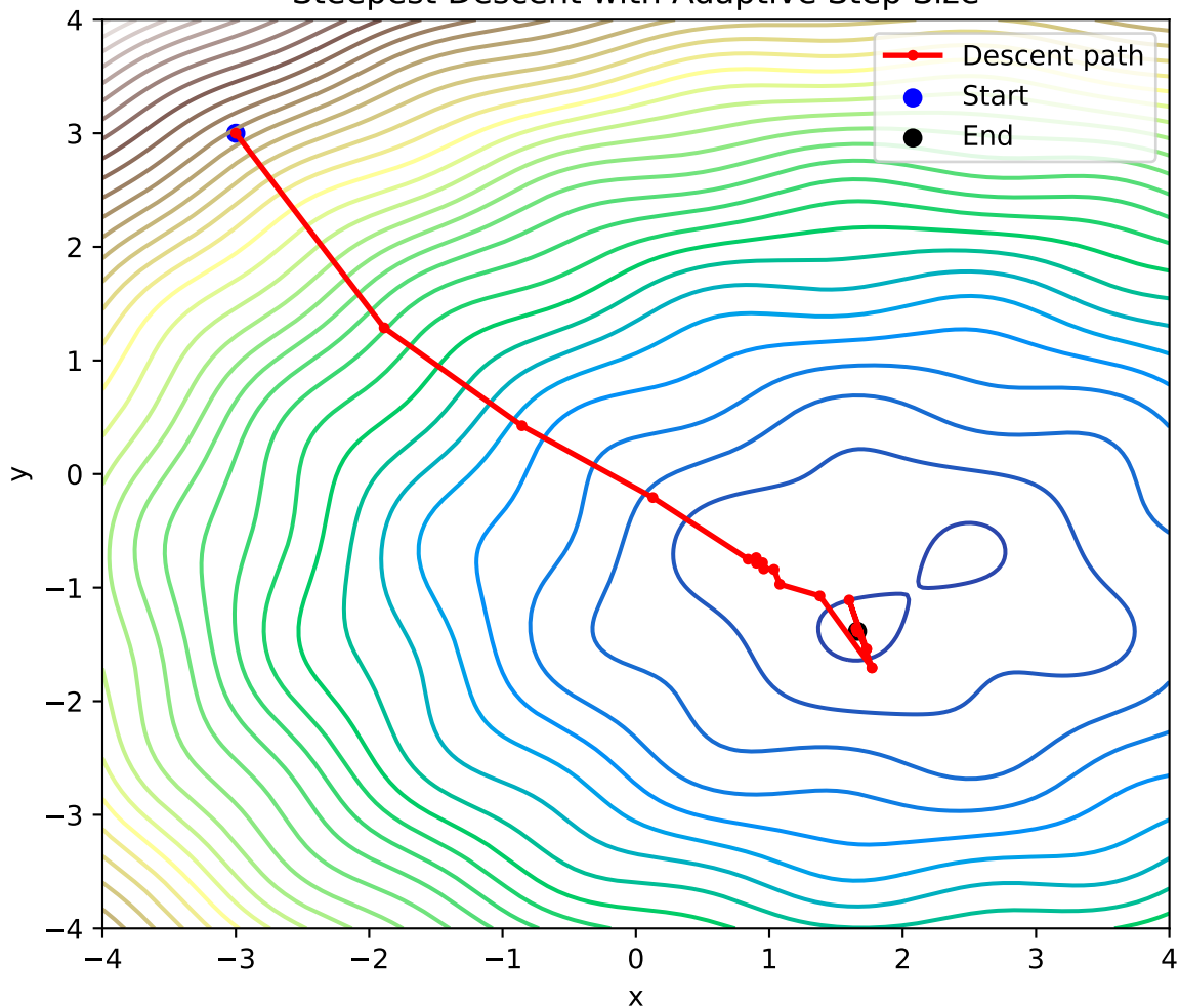
Steepest Descent with Adaptive Step Size
