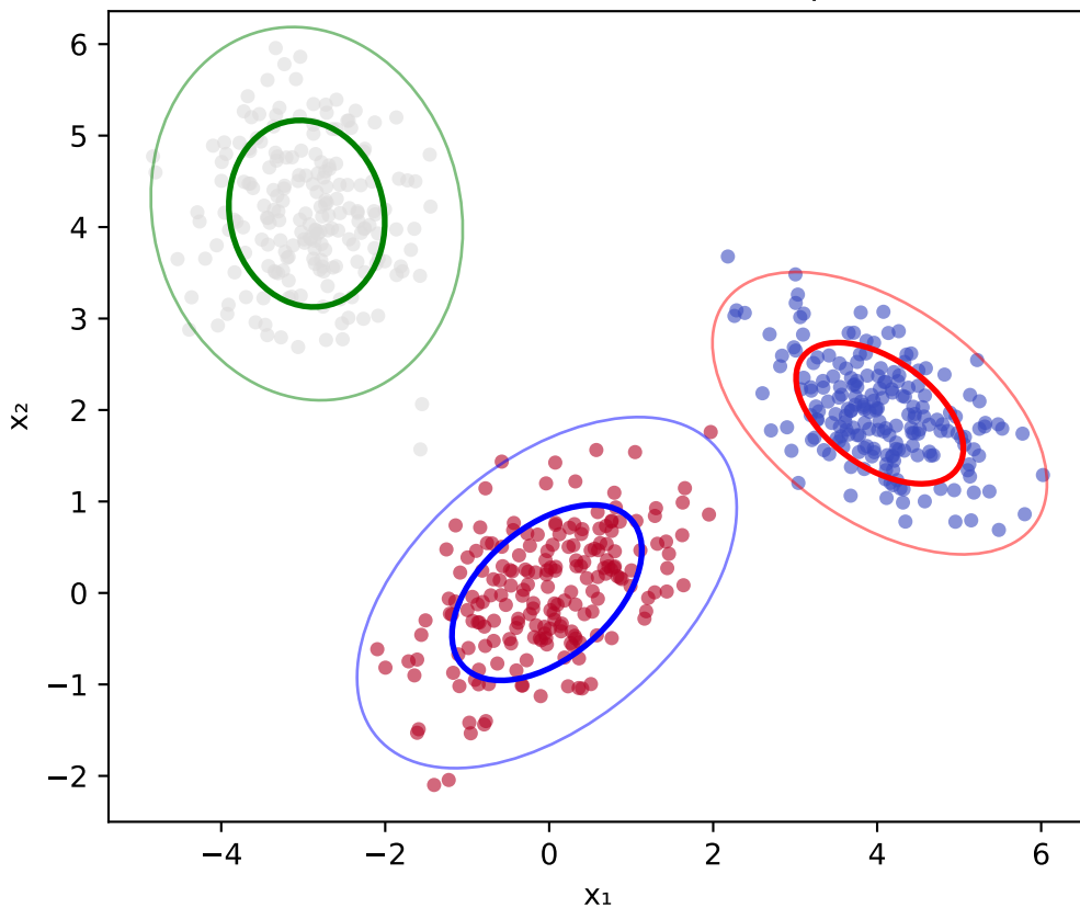
Gaussian Mixture Model fit to a 2D point cloud
