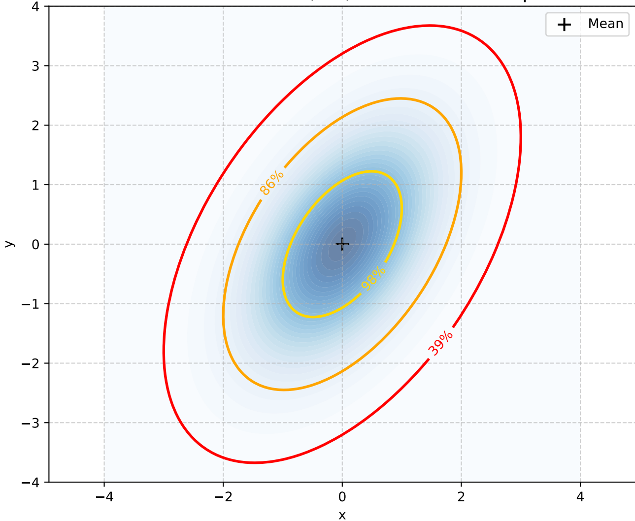
2D Gaussian with 1\sigma , 2\sigma , 3\sigma Confidence Ellipses
