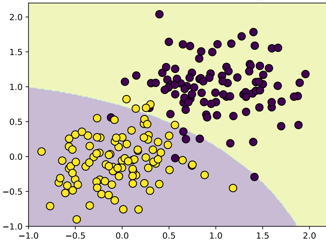
Gaussian Mixture Models decision regions
