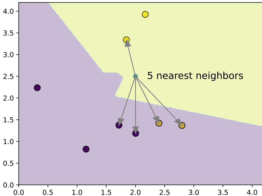
5-NN classification regions
