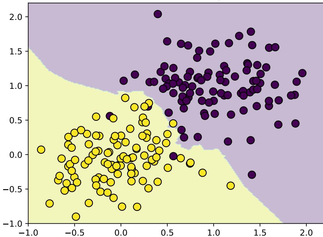
5-NN classification regions
