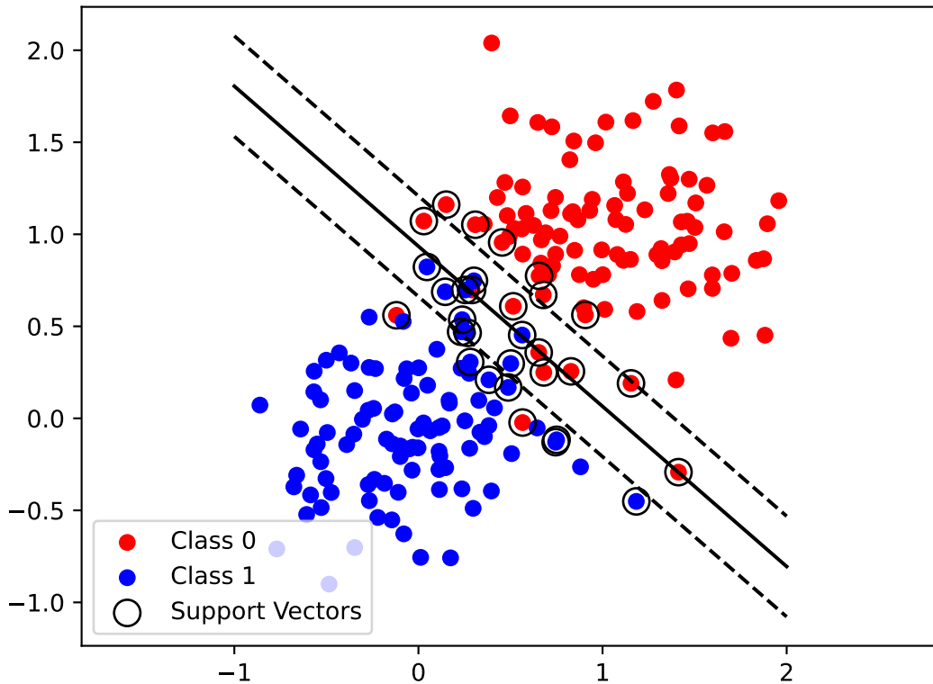
Linear SVM with explicit w \cdot x + b = 0 boundary
