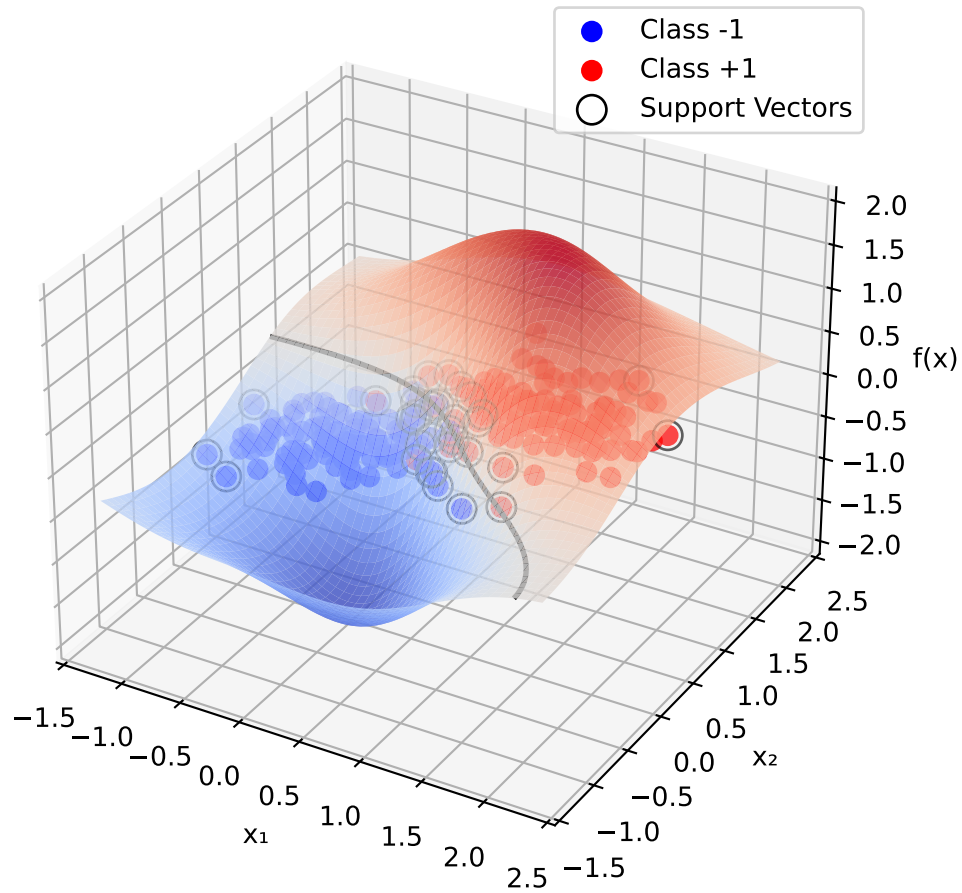
RBF SVM decision surface
