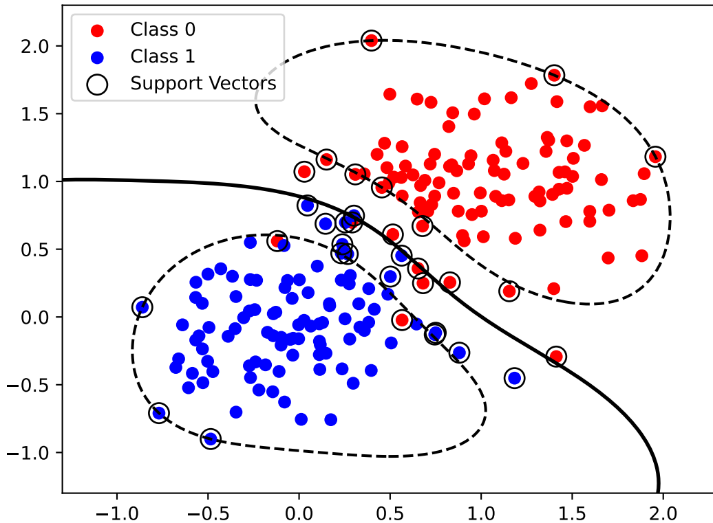
SVM Decision Boundary and Support Vectors
