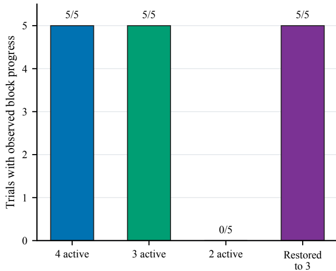
Crash-fault liveness boundary
