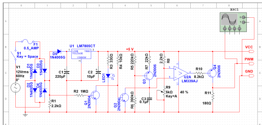
Figure 1: Programmable Pulse Generator
