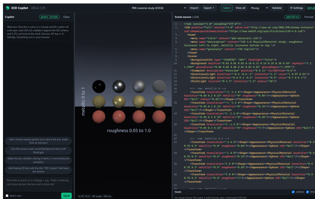
Figure 1: Left: the three panes – copilot chat, X_ITE view, source with inline diagnostics (PBR material study, X3D 4.0 PhysicalMaterial). Right: a selected Transform with the X3D-native gizmo and the inspector; the edited attributes are highlighted in the source.
