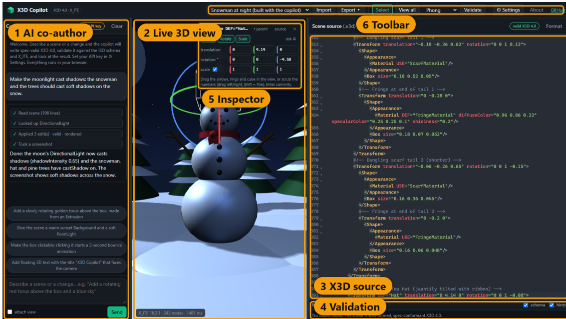
Figure 1: The interface, with the copilot-authored snowman example loaded and its hat selected. (1) AI co-author: the conversation with the model; each tool call appears as a step that can be expanded to show the validation report the model received. (2) Live 3D view: X_ITE renders the scene as the source changes; clicking geometry selects it. (3) X3D source: a code editor with specification-driven autocompletion and inline diagnostics. (4) Validation: findings of the three validators, with jump-to-line. (5) Inspector: translation, rotation and scale of the selected object, editable, synchronised with the source and passed to the model as context. (6) Toolbar: examples, import, export, shading, view control and model settings.
