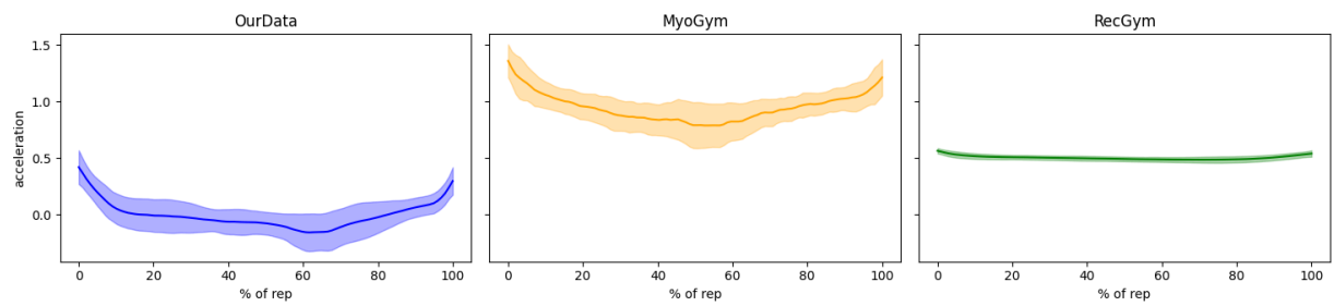
Bench Press for y_accel
