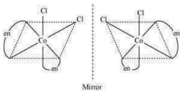
Optical isomers of \text{cis-}[\text{CoCl}_2(\text{en})_2]^+ - part (i)
