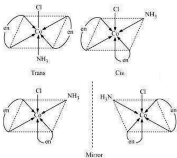
Trans and cis isomers of [\text{Co}(\text{NH}_3)\text{Cl}(\text{en})_2]^{2+} - part (ii)
