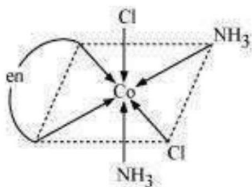
Geometrical isomer of [\text{Co}(\text{NH}_3)_2\text{Cl}_2(\text{en})]^+ - part (iii)
