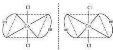
Optical isomers of \text{trans-}[\text{CoCl}_2(\text{en})_2]^+ - part (i)
