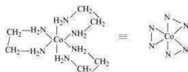
Two optical isomers of [\text{Co}(\text{en})_3]\text{Cl}_3
