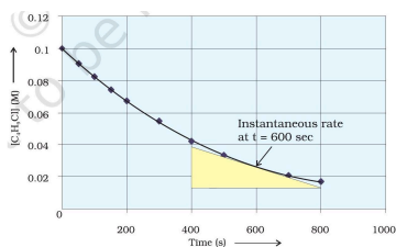
Fig 3.2 Instantaneous rate of hydrolysis of butyl chloride ( \text{C}_4\text{H}_9\text{Cl} )
