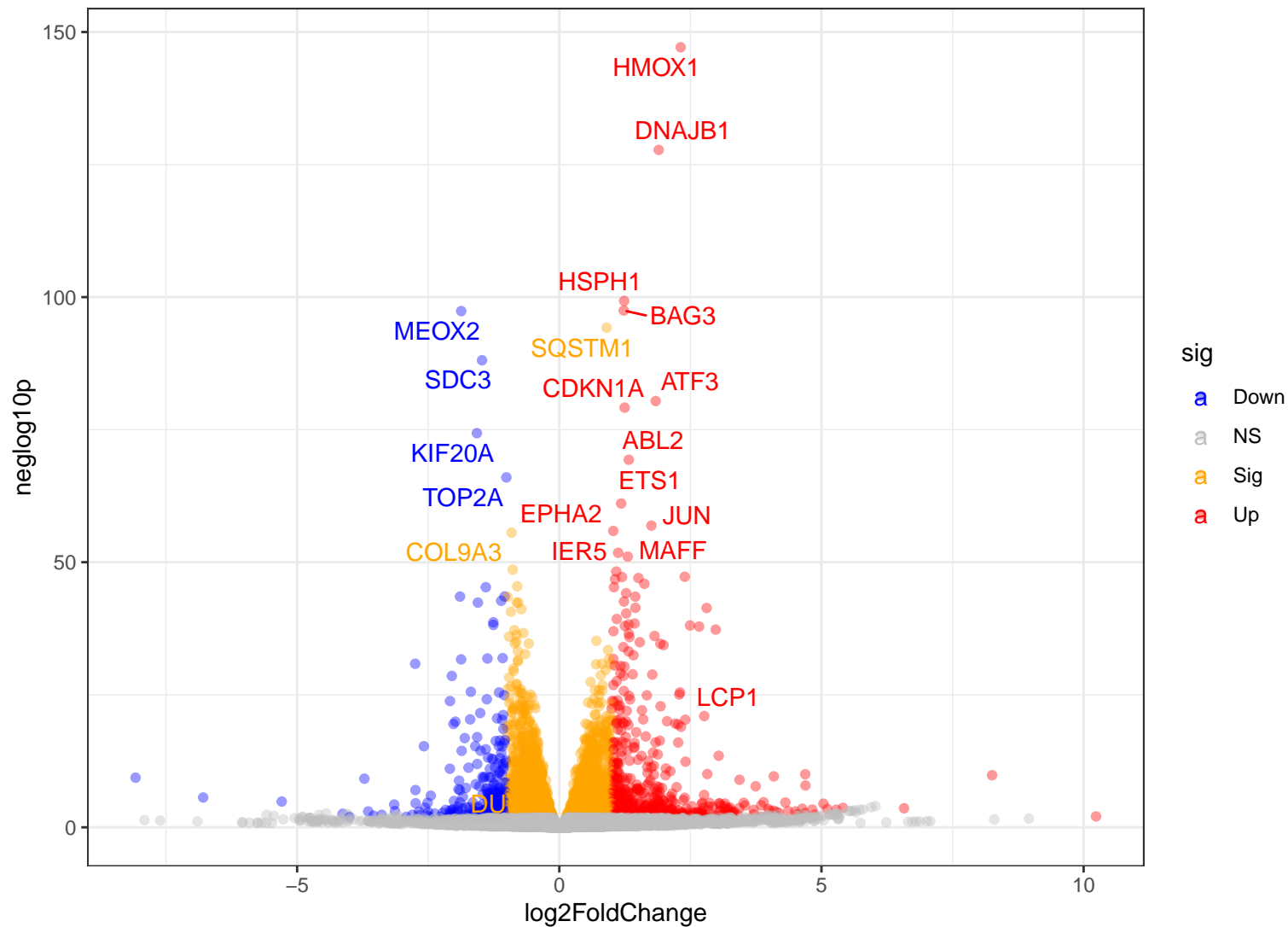
Volcano Plot: KO vs WT
