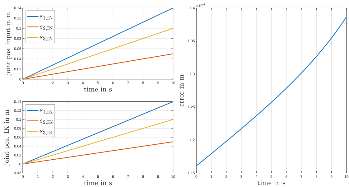
Figure 3.2: Plot of Verification process for inverse kinematics. Left column: input joint position into Multibody model (MB) and output of inverse kinematics function (IK); right column: euclidean error of the two
