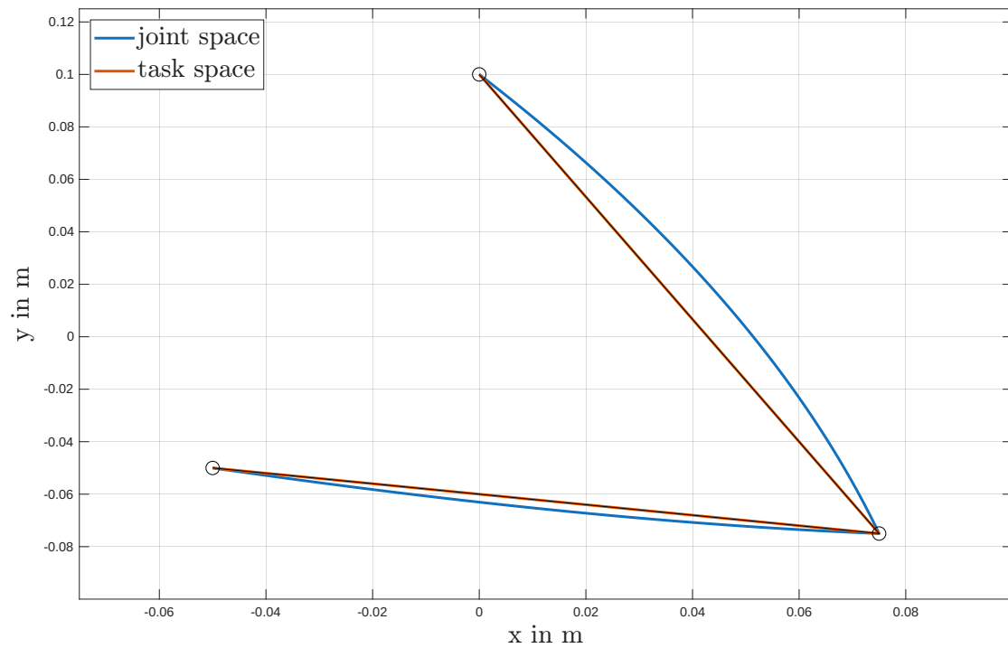
Figure 5.3: End-effector position in joint and task space
