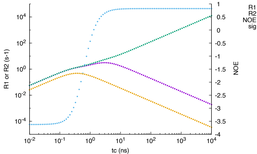
Isotropic model, local residue timescale fit
