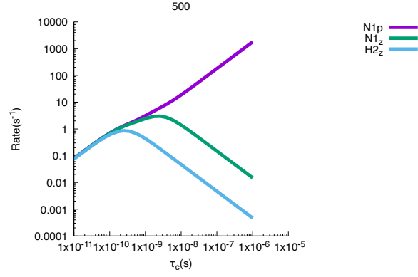
Figure 1: Relaxation rates versus correlation time \tau_c for spin system NH. macro=False. \nu_0 500.00 MHz. AXIAL DIFFUSION: Rotation into diffusion frame, \theta_O 0.25\pi , \phi_O 1.00\pi , shape factor, 1.00\text{e}+01 ns. \tau_{\parallel} 4.00\text{e}+01 ns. \beta=0.00^\circ ( P rank 2). =0.00^\circ ( Q rank 2). Dipolar d : (\gamma_N, \gamma_H) , R_d=1.02\text{\AA} , d=7.21\text{e}+04 rad s -2 . CSA: c_A ( \gamma_N ) -160.00ppm, c_A=1.70\text{e}+04 rad s -2 . CSA: c_X ( \gamma_H ) 10.00ppm, c_X=1.05\text{e}+04 rad s -2 .
