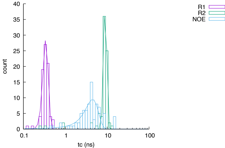
Isotropic model, local timescale fit
