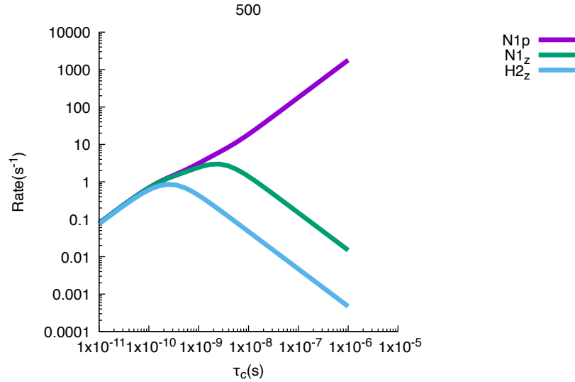
Figure 1: Relaxation rates versus correlation time \tau_c for spin system NH. macro=False. \nu_0 500.00 MHz. AXIAL DIFFUSION: Rotation into diffusion frame, \theta_O 0.25 \pi , \phi_O 1.00 \pi , shape factor, 1.00e+01 ns. \tau_{||} 4.00e+01 ns. \beta=0.00^\circ ( P rank 2). =0.00^\circ ( Q rank 2). Dipolar d : ( \gamma_N , \gamma_H ), R_d=1.02\text{\AA} , d=7.21e+04 rad s -2 . CSA: c_A ( \gamma_N ) -160.00ppm, c_A=1.70e+04 rad s -2 . CSA: c_X ( \gamma_H ) 10.00ppm, c_X=1.05e+04 rad s -2 .
