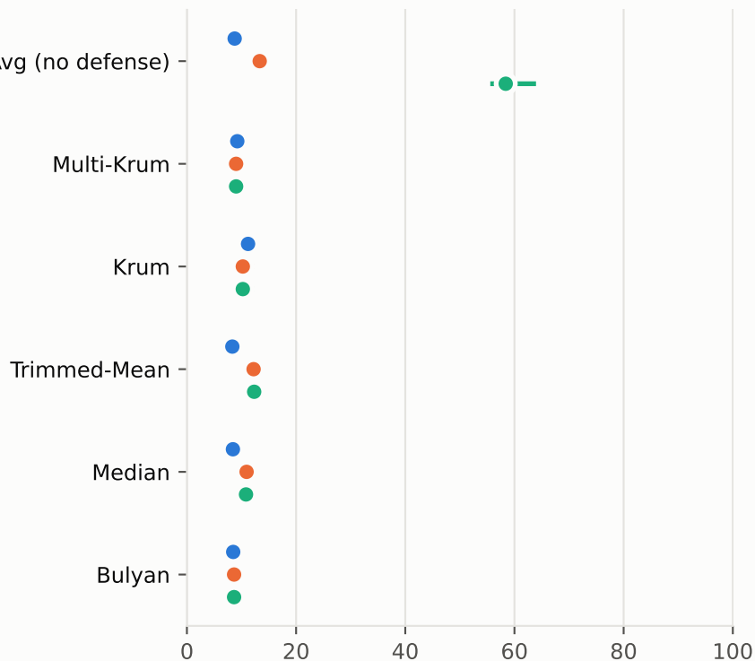
Attack success, mean of rounds 6-20 (%)
