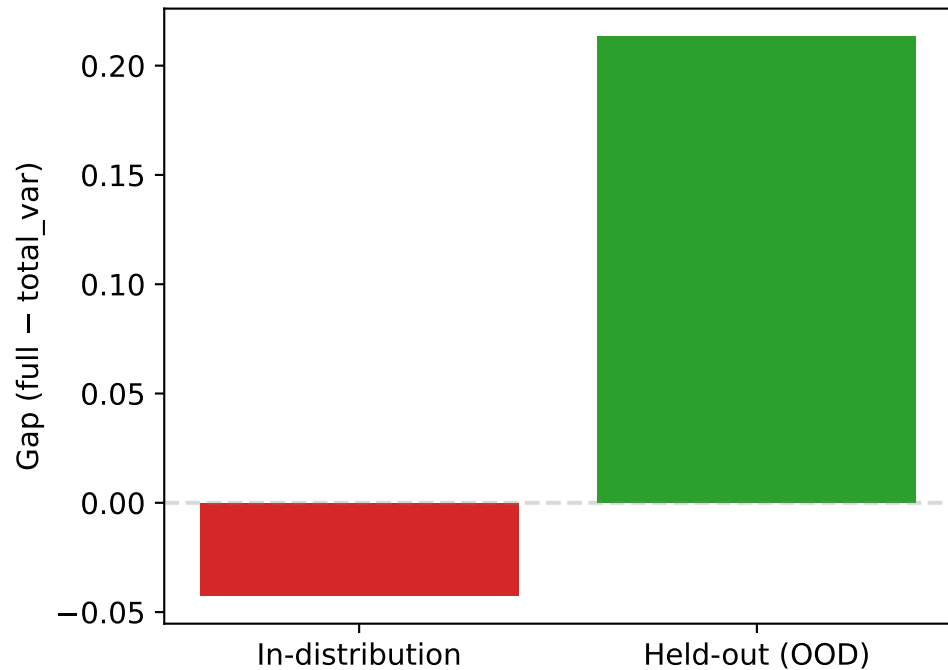
Decomposition gap widens under OOD
