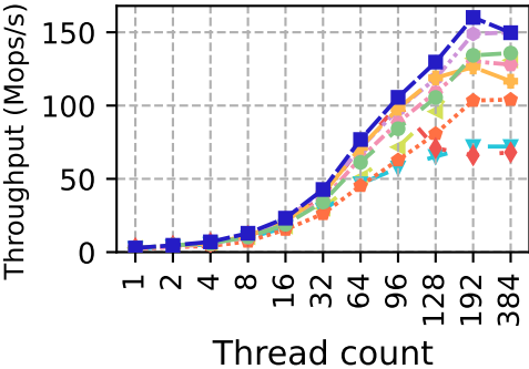
skip-list
