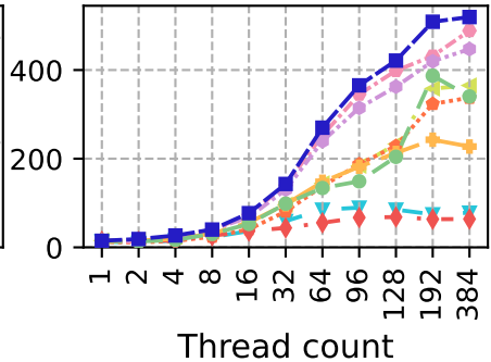
hash-block
