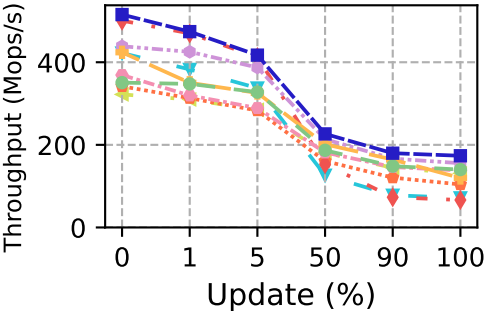
skip-list
