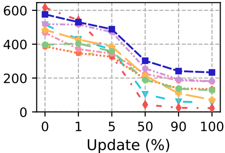
leaf-tree
