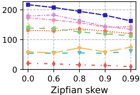
leaf-tree
