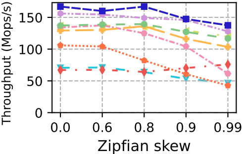
skip-list
