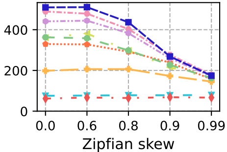
hash-block
