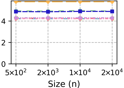
hmlist
