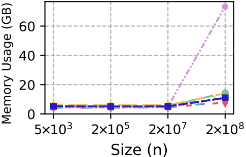
bst-tk
