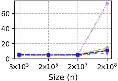
abtree
