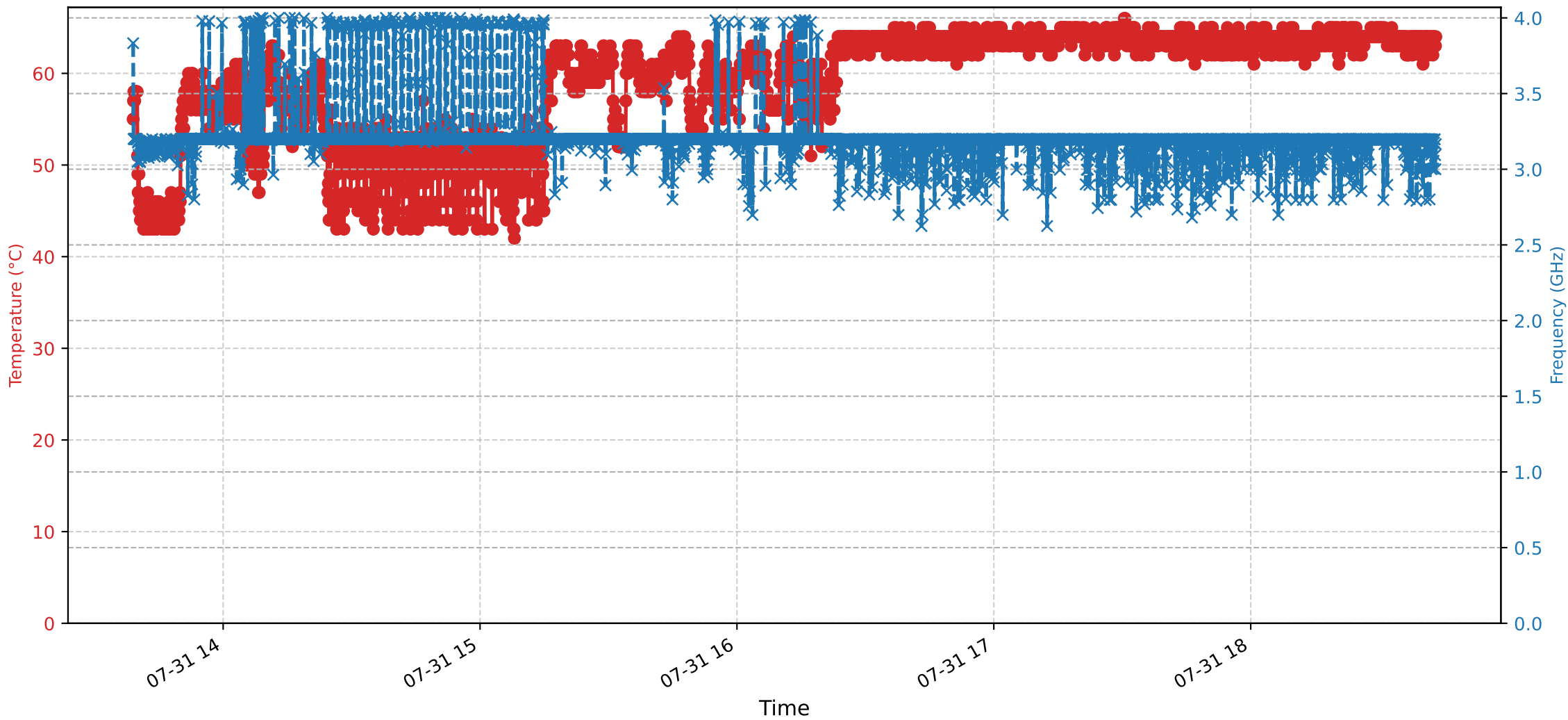
Device Temperature and Frequency over Time
