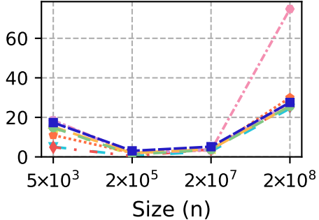
hash-block
