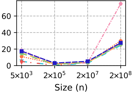
leaf-tree
