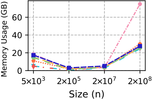
skip-list
