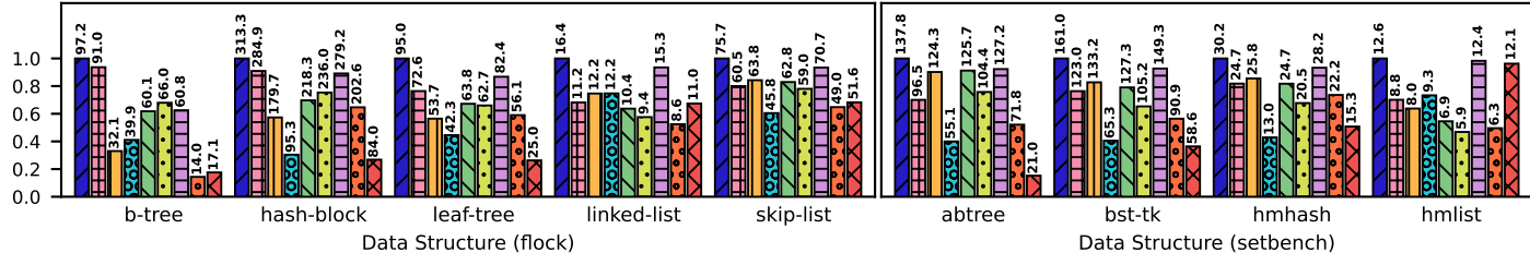
Normalized Geomean Throughput (Mops/s)
