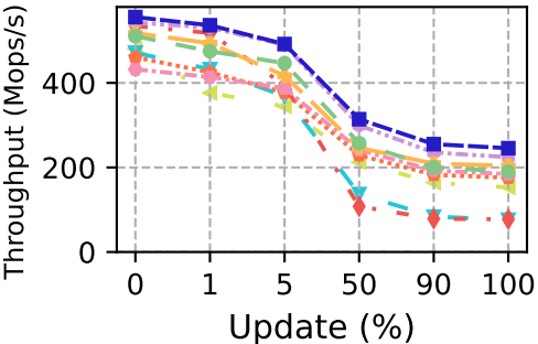
bst-tk
