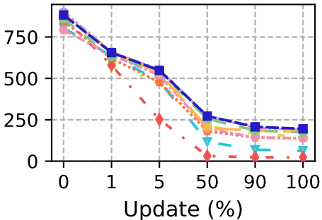
abtree
