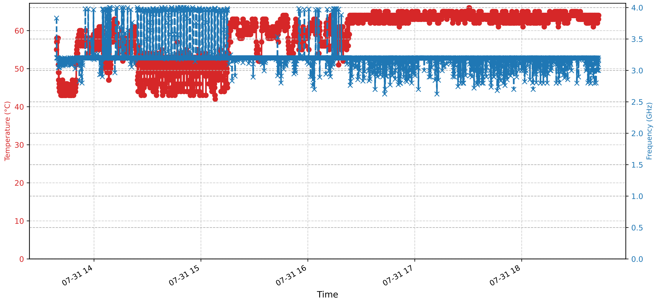
Device Temperature and Frequency over Time
