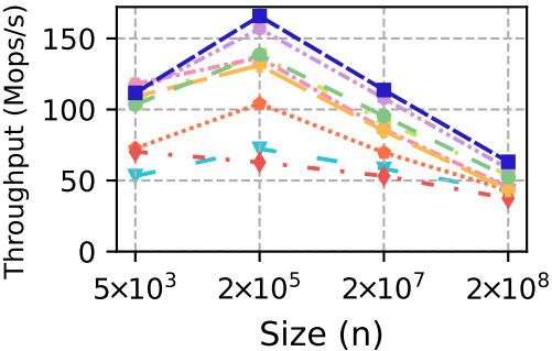
skip-list
