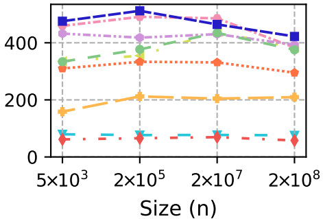
hash-block
