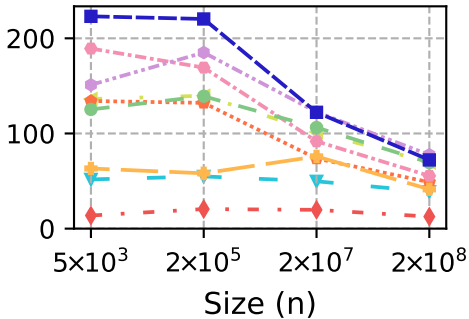
leaf-tree
