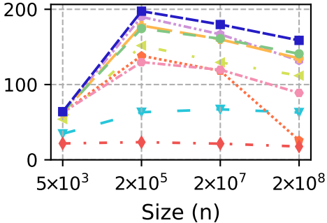
abtree
