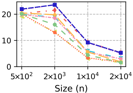
hmlist
