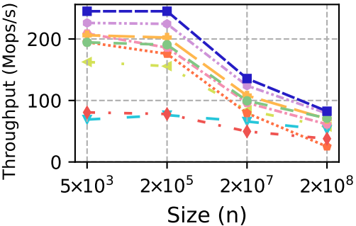
bst-tk
