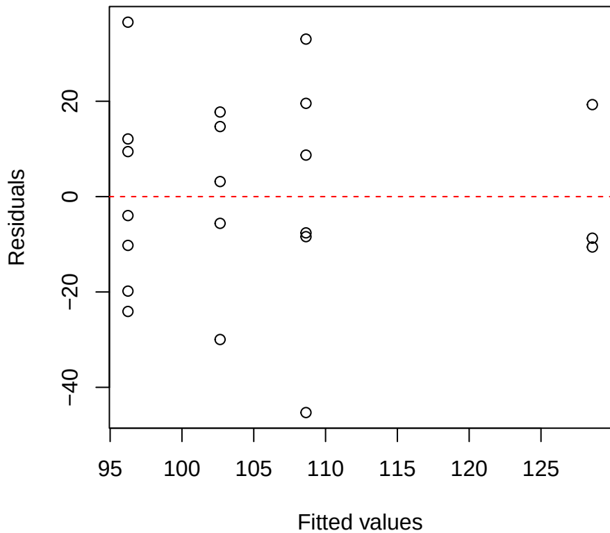
iWUE | 3000 | Hedyosmum Residuals vs Fitted
