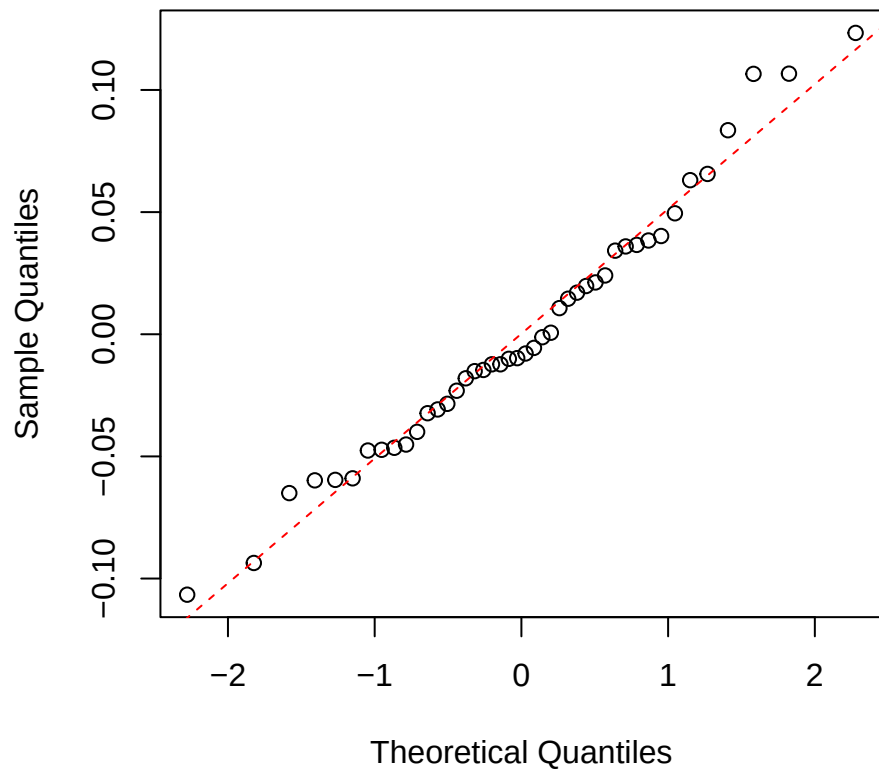
Thickness | 2000 | Alchornea Normal Q-Q
