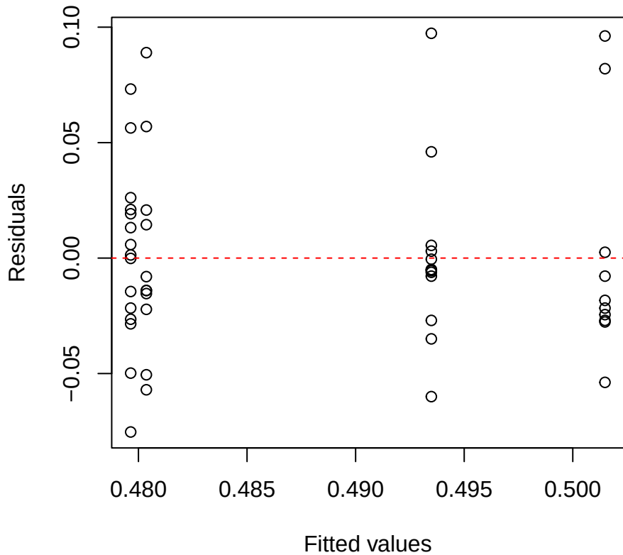
Thickness | 2000 | Myrcia Residuals vs Fitted
