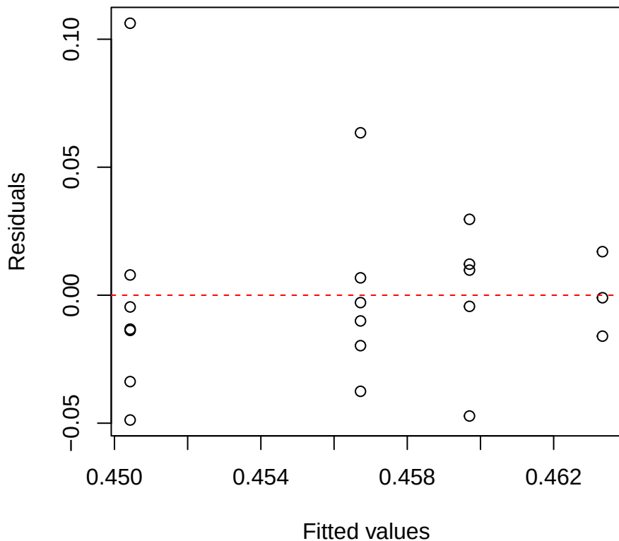
Thickness | 3000 | Hedyosmum Residuals vs Fitted
