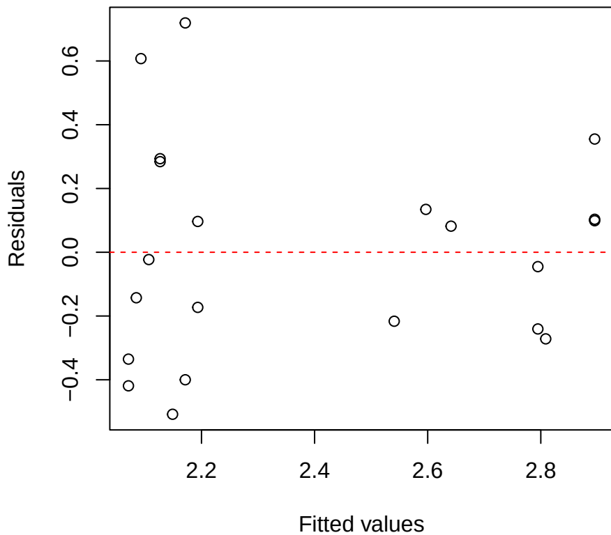
Narea | 3000 | Hedyosmum Residuals vs Fitted
