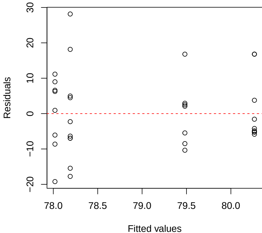
SLA | 1000 | Pouteria Residuals vs Fitted
