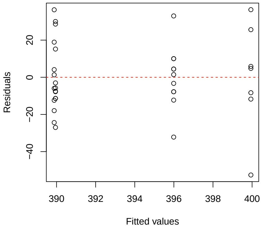
Ci | 1000 | Pouteria Residuals vs Fitted
