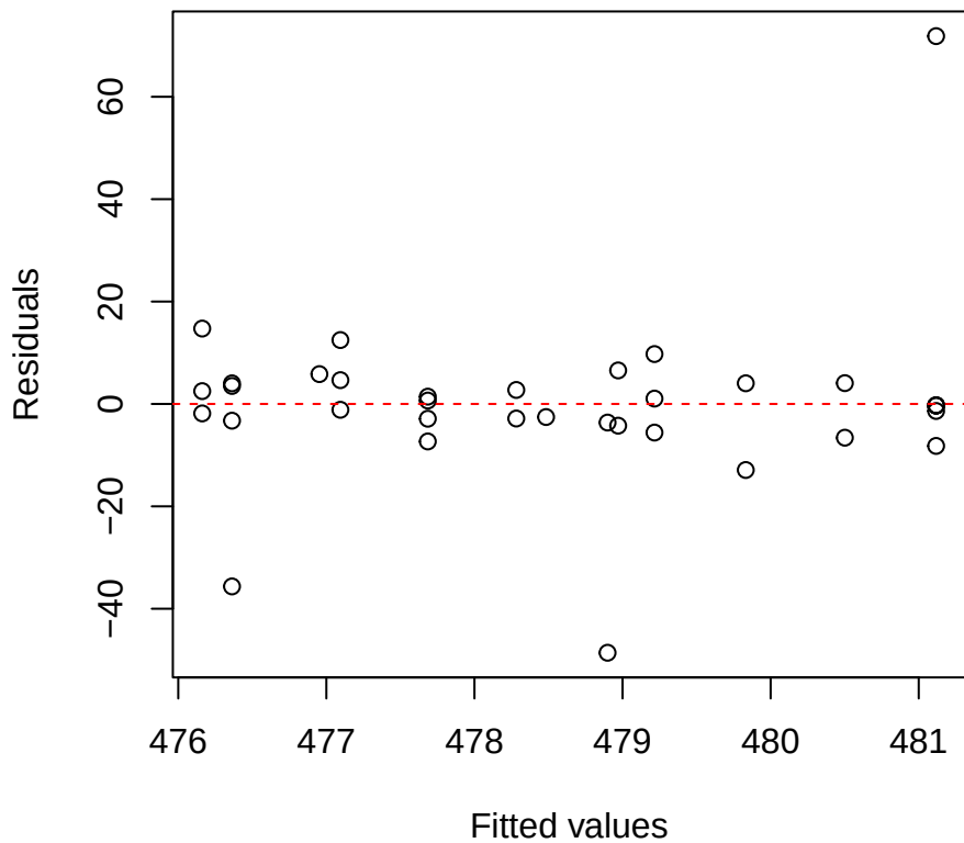
Cmass | 1000 | Pouteria Residuals vs Fitted
