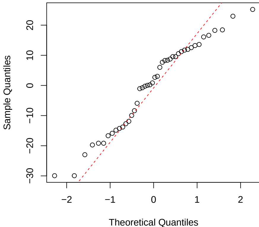
iWUE | 2000 | Alchornea Normal Q-Q
