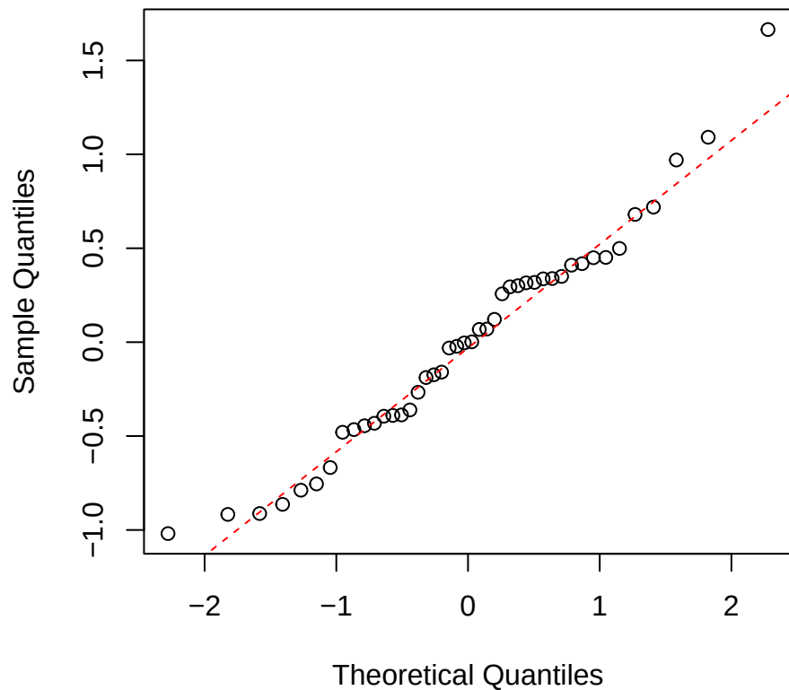
Narea | 2000 | Alchornea Normal Q-Q
