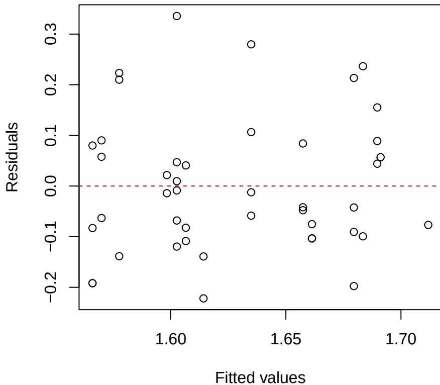
Toughness | 2000 | Alchornea Residuals vs Fitted
