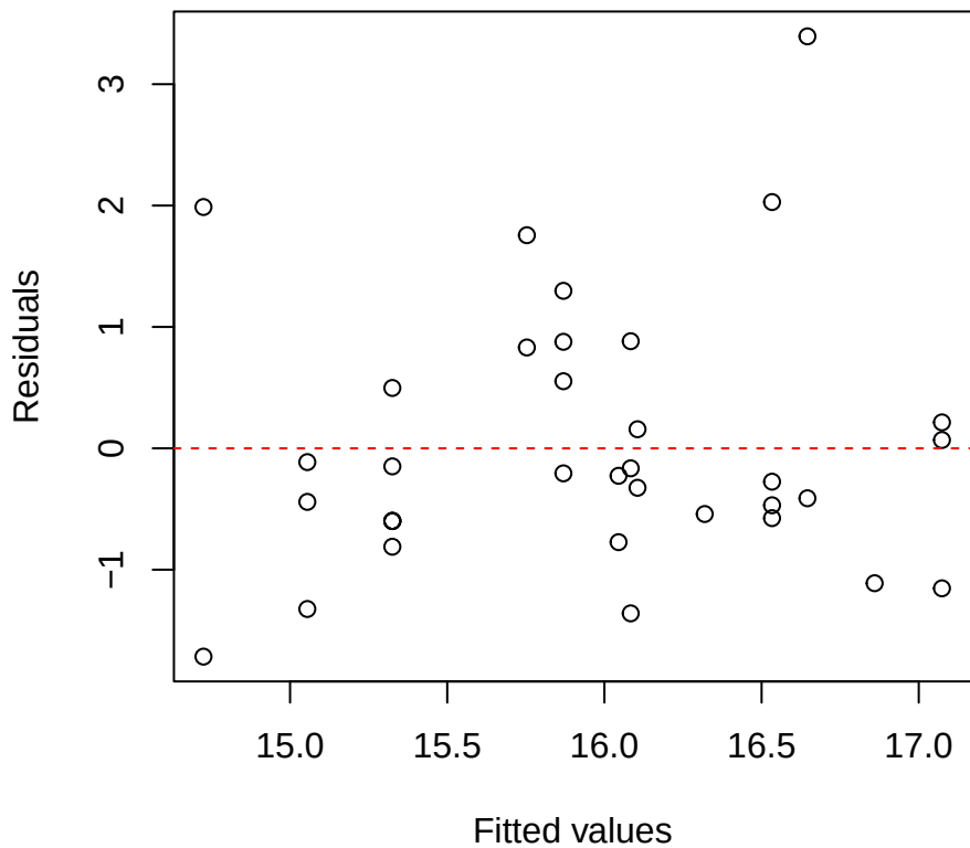
Nmass | 1000 | Pouteria Residuals vs Fitted
