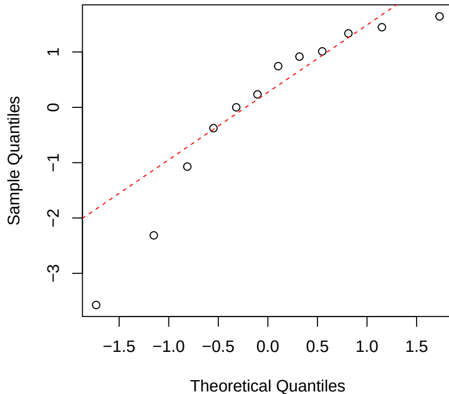
Carea | 1000 | Clarisia Normal Q-Q
