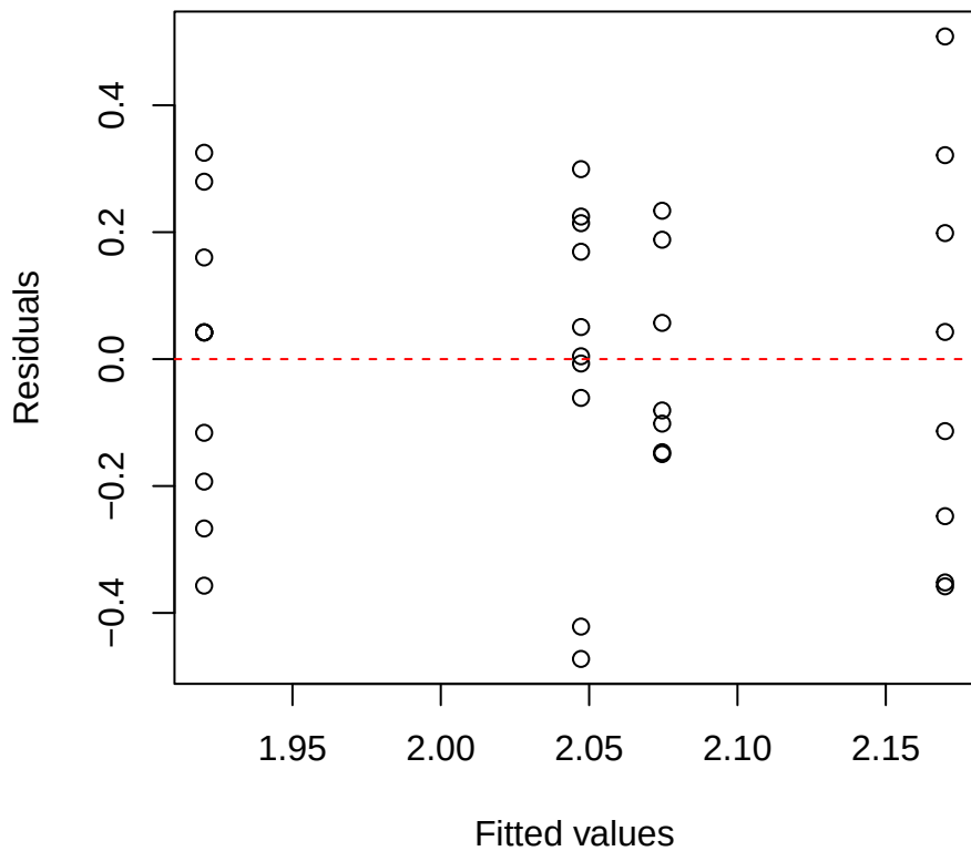
Narea | 1000 | Pouteria Residuals vs Fitted
