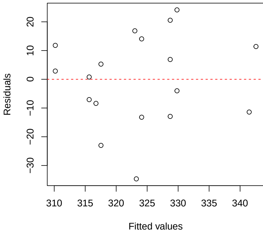
Ci | 3000 | Weinmannia Residuals vs Fitted
