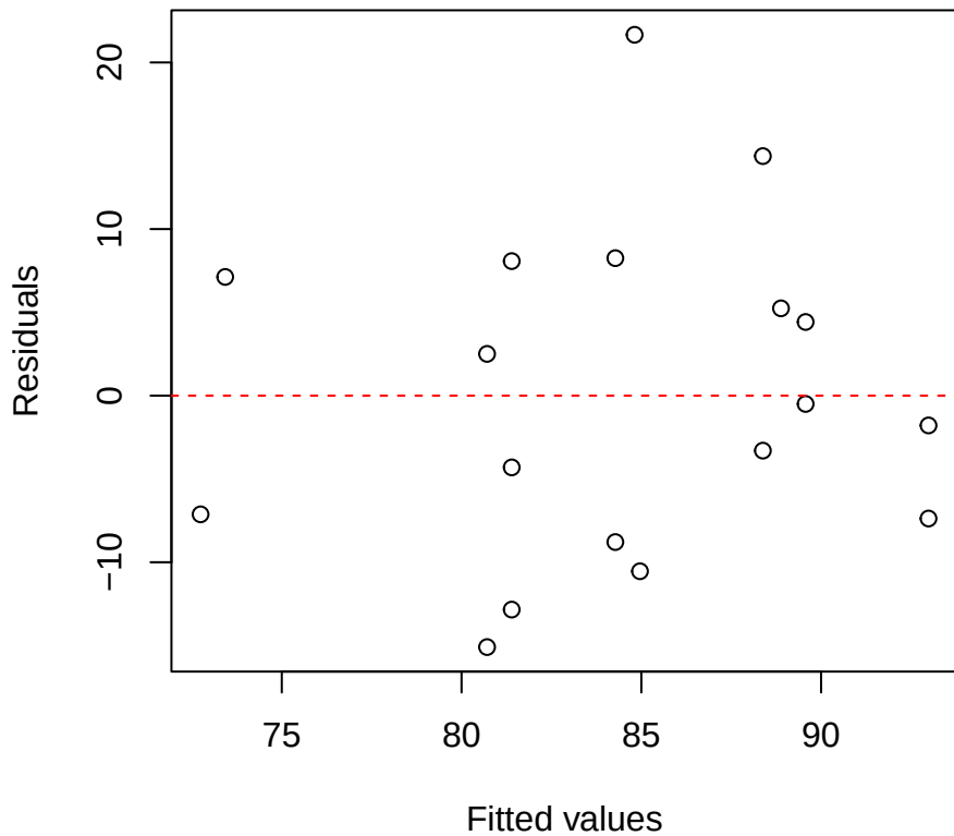
iWUE | 3000 | Weinmannia Residuals vs Fitted
