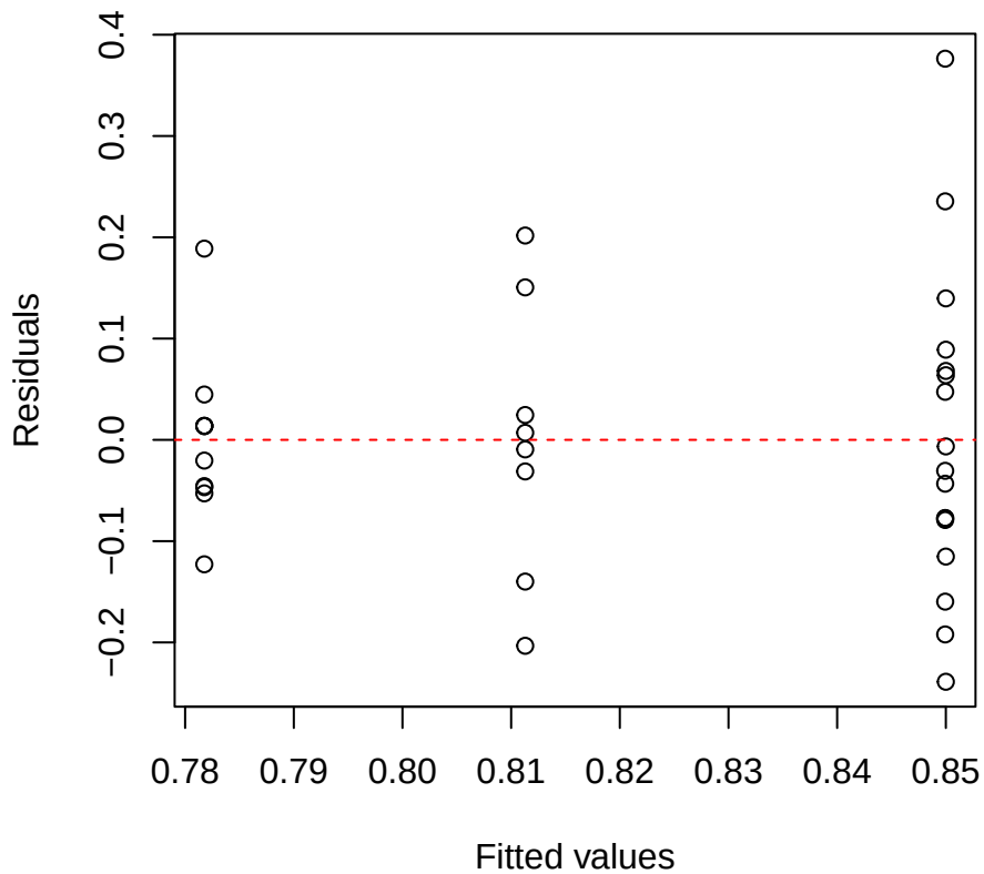
Toughness | 1000 | Pouteria Residuals vs Fitted
