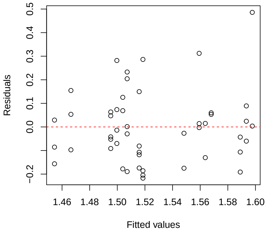
Toughness | 2000 | Myrcia Residuals vs Fitted
