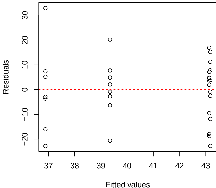
iWUE | 1000 | Pouteria Residuals vs Fitted
