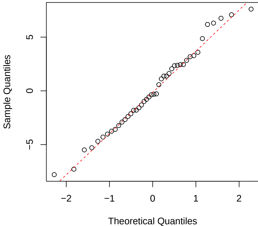
SLA | 2000 | Alchornea Normal Q-Q
