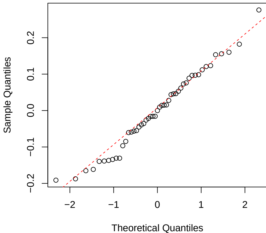
logNmass | 2000 | Myrcia Normal Q-Q
