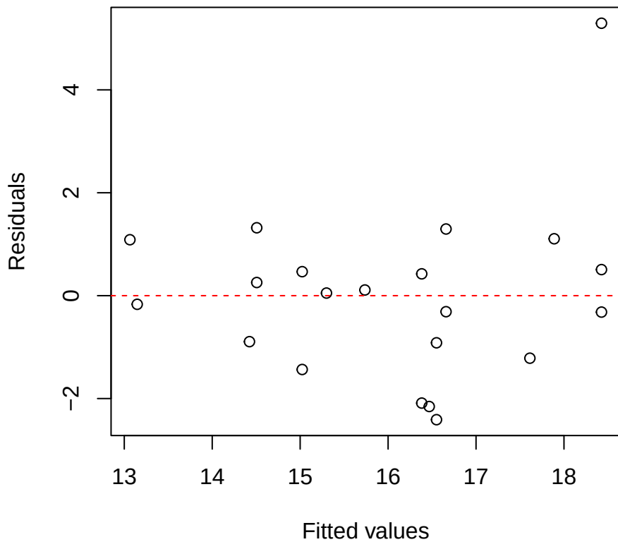
Nmass | 3000 | Hedyosmum Residuals vs Fitted
