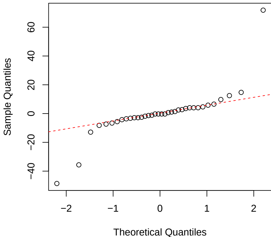
Cmass | 1000 | Pouteria Normal Q-Q
