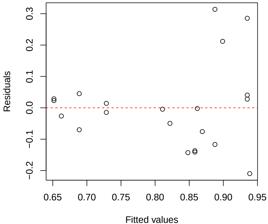
Toughness | 3000 | Hedyosmum Residuals vs Fitted
