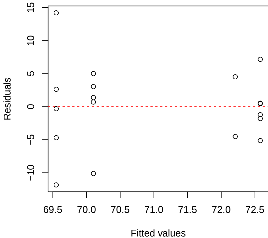
SLA | 3000 | Weinmannia Residuals vs Fitted
