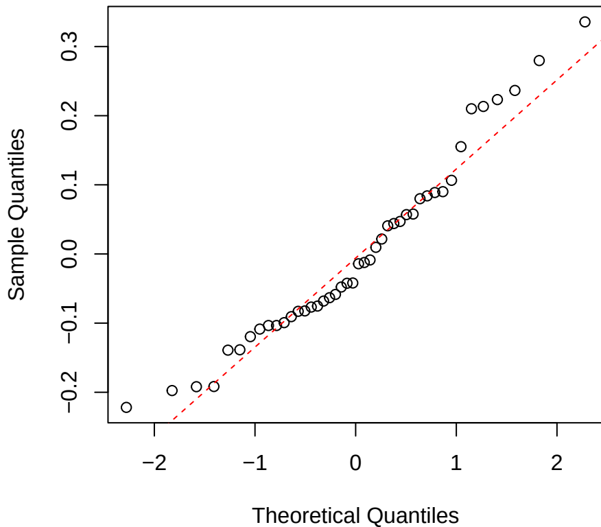
Toughness | 2000 | Alchornea Normal Q-Q
