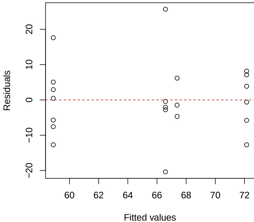
Carea | 3000 | Hedyosmum Residuals vs Fitted
