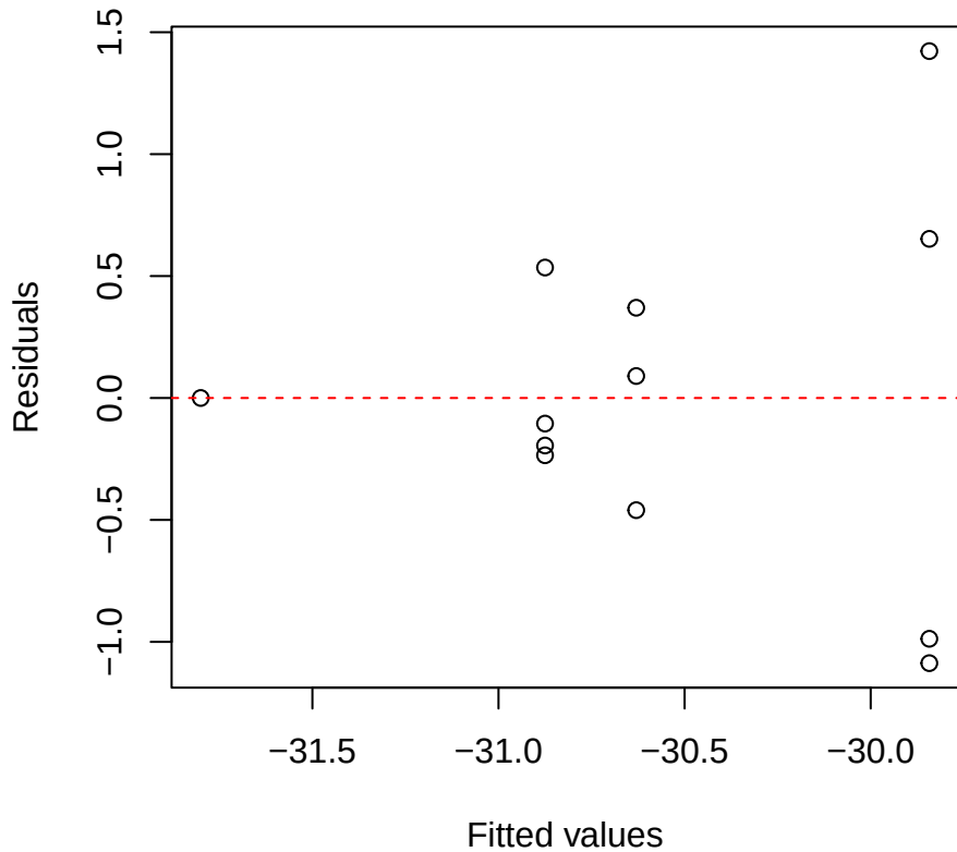
d13C | 1000 | Clarisia Residuals vs Fitted
