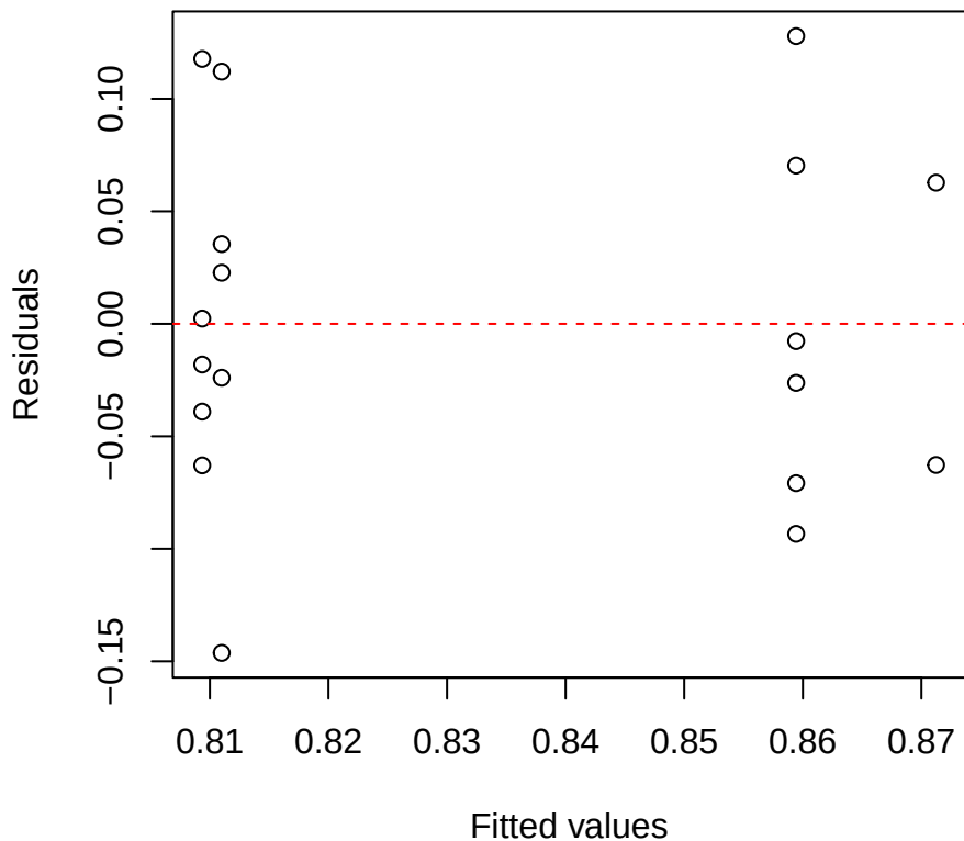
Toughness | 3000 | Weinmannia Residuals vs Fitted
