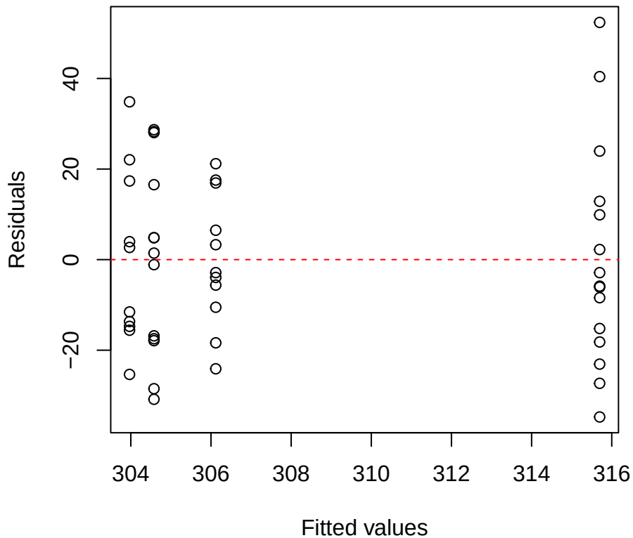
Ci | 2000 | Myrcia Residuals vs Fitted
