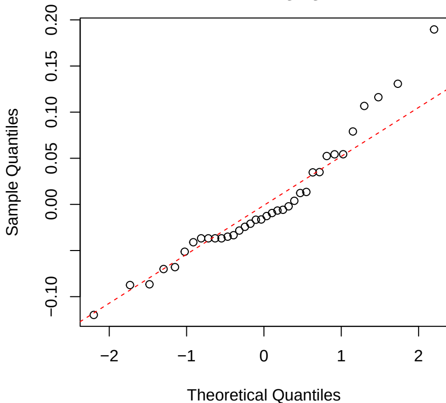
logNmass | 1000 | Pouteria Normal Q-Q
