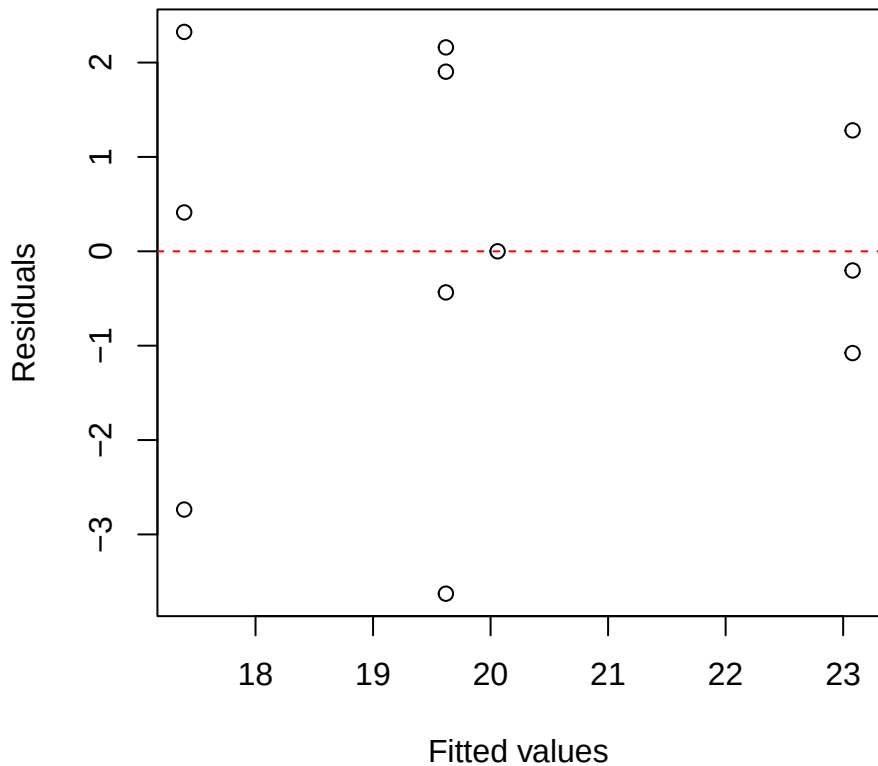
Nmass | 1000 | Clarisia Residuals vs Fitted
