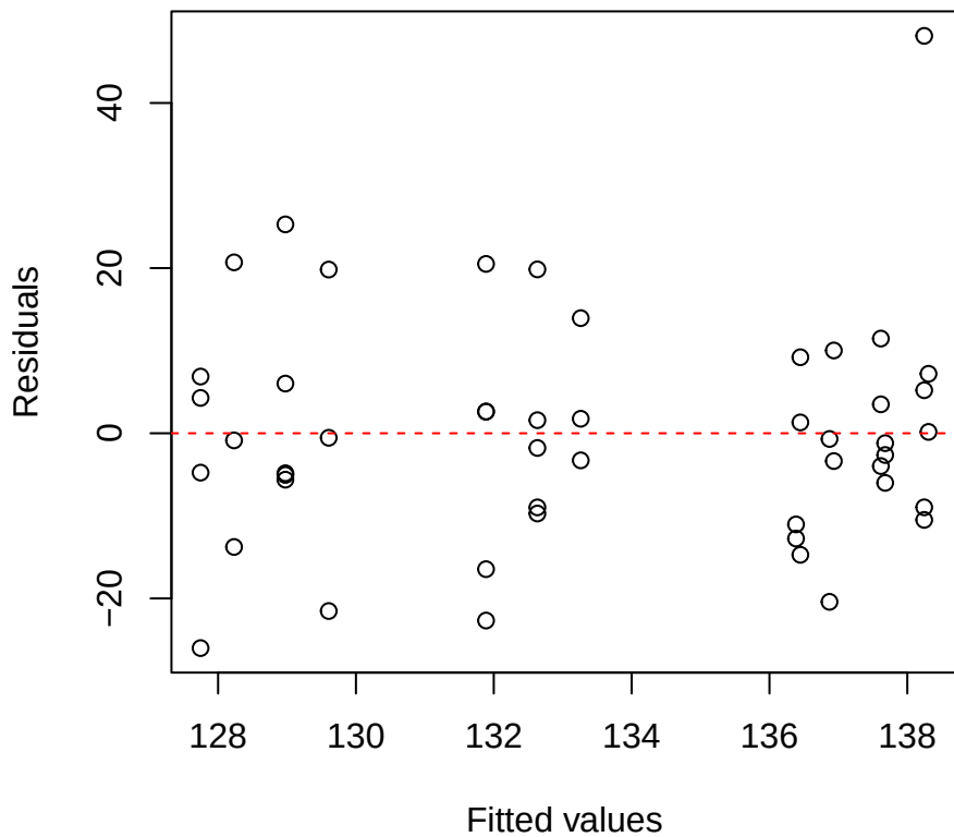
Carea | 2000 | Myrcia Residuals vs Fitted
