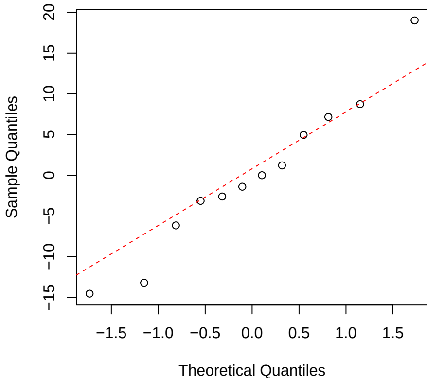
iWUE | 1000 | Clarisia Normal Q-Q
