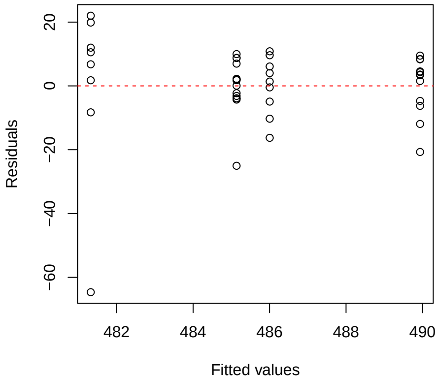
Cmass | 2000 | Alchornea Residuals vs Fitted
