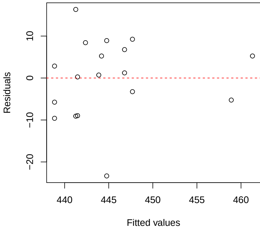
Cmass | 3000 | Weinmannia Residuals vs Fitted
