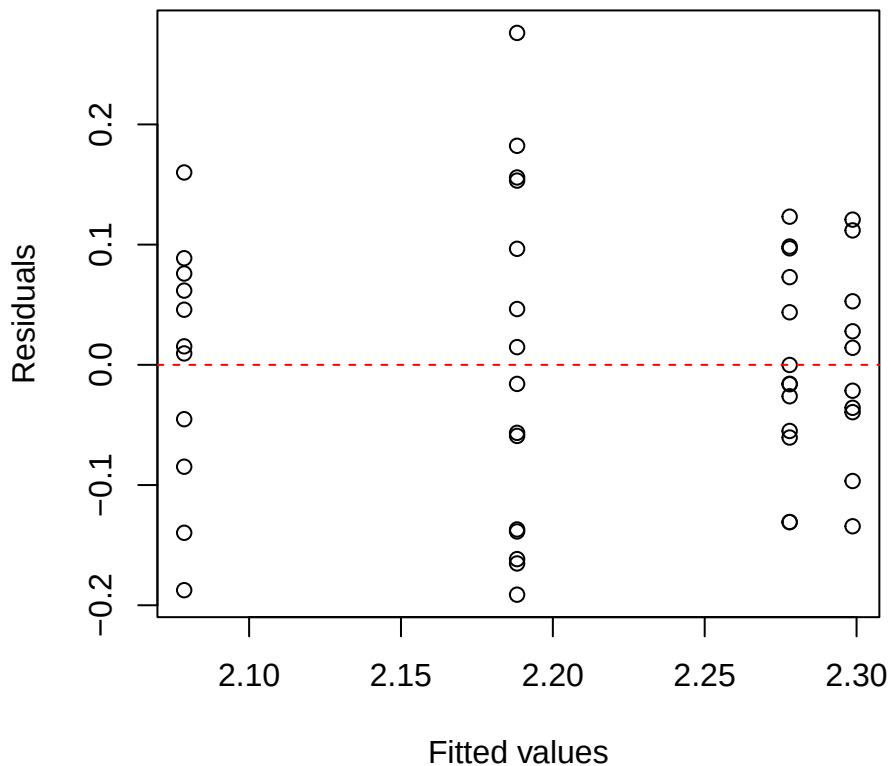
logNmass | 2000 | Myrcia Residuals vs Fitted
