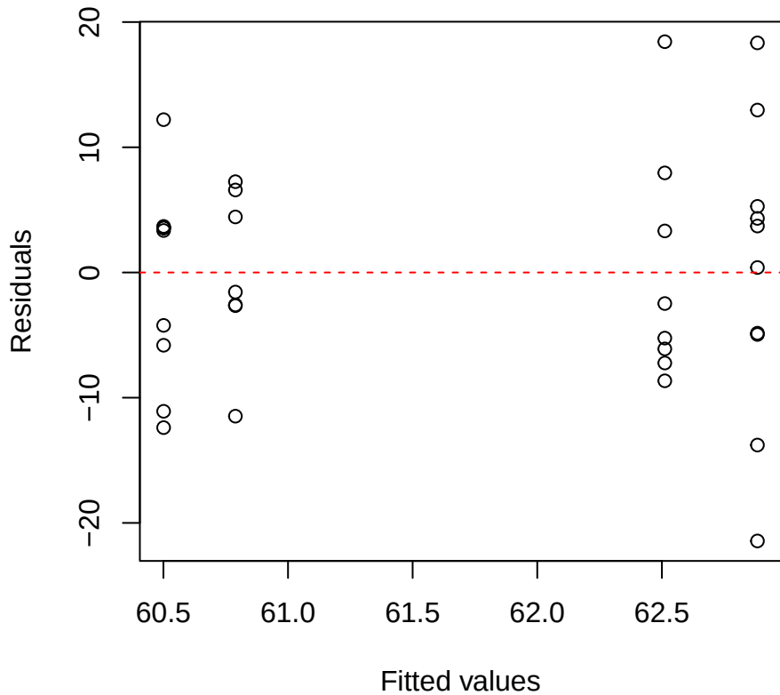
Carea | 1000 | Pouteria Residuals vs Fitted
