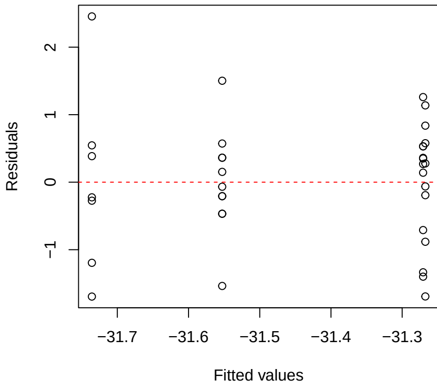
d13C | 1000 | Pouteria Residuals vs Fitted
