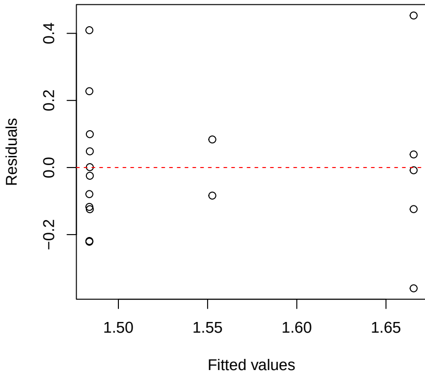
Narea | 3000 | Weinmannia Residuals vs Fitted
