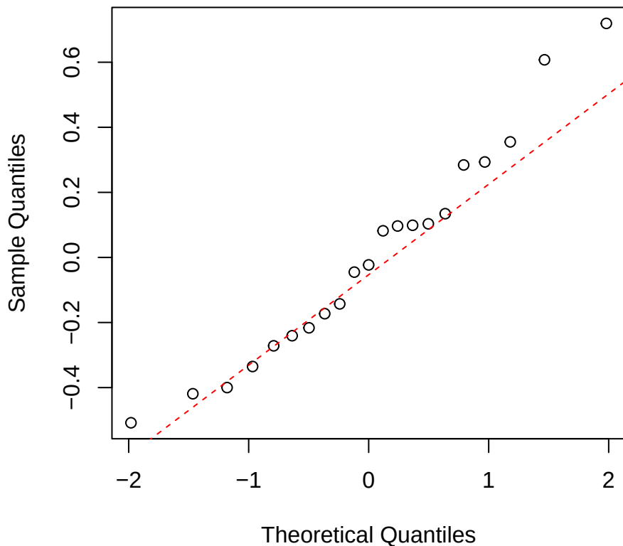
Narea | 3000 | Hedyosmum Normal Q-Q
