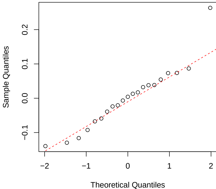
logNmass | 3000 | Hedyosmum Normal Q-Q
