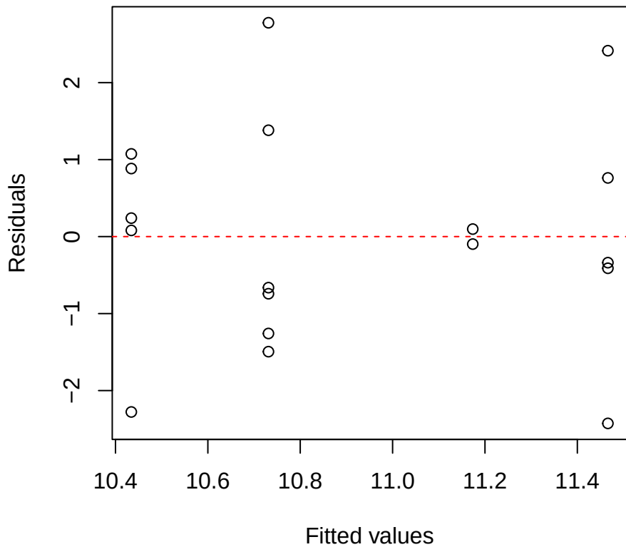
Nmass | 3000 | Weinmannia Residuals vs Fitted
