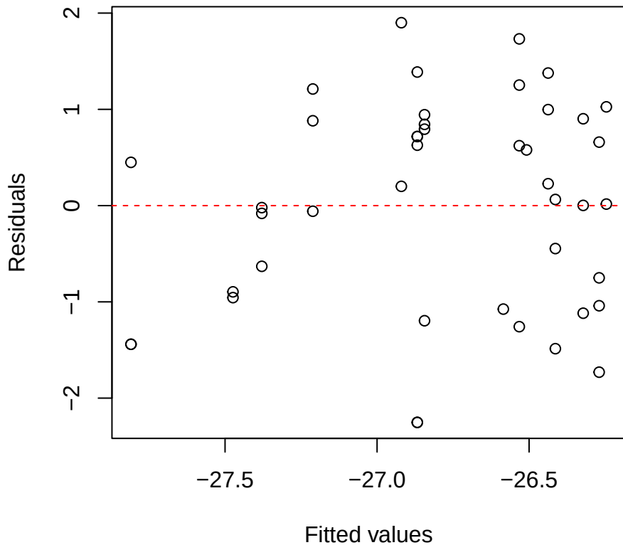
d13C | 2000 | Alchornea Residuals vs Fitted
