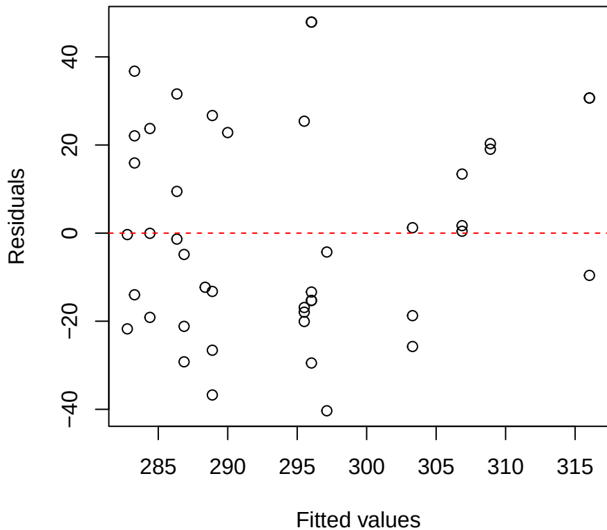
Ci | 2000 | Alchornea Residuals vs Fitted
