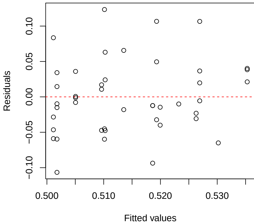
Thickness | 2000 | Alchornea Residuals vs Fitted
