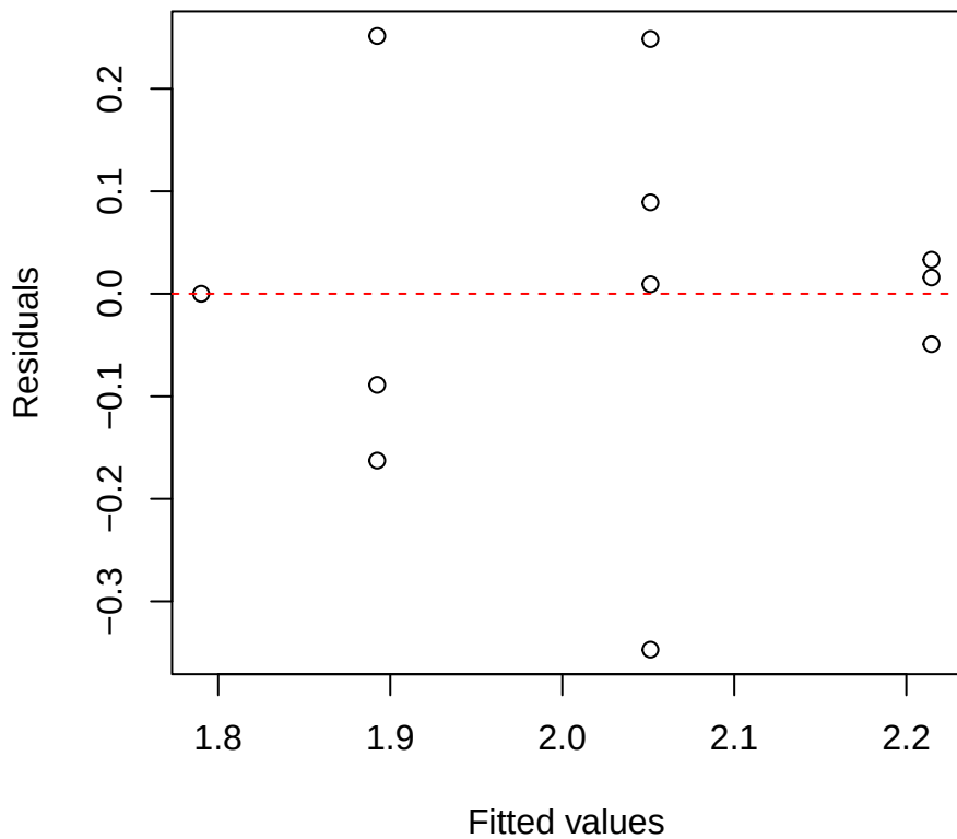
Narea | 1000 | Clarisia Residuals vs Fitted
