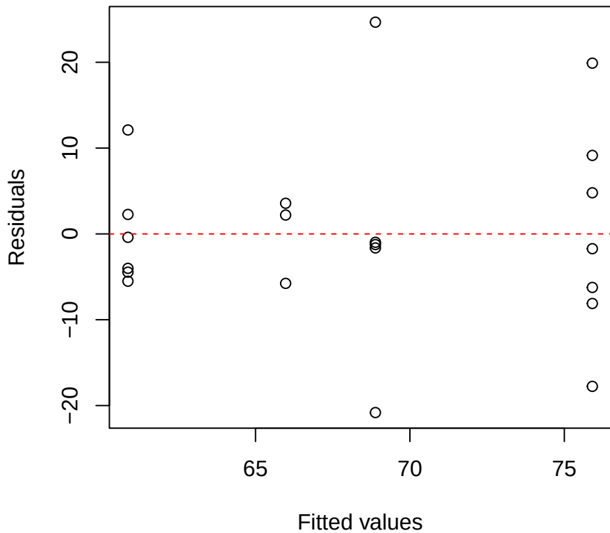
SLA | 3000 | Hedyosmum Residuals vs Fitted
