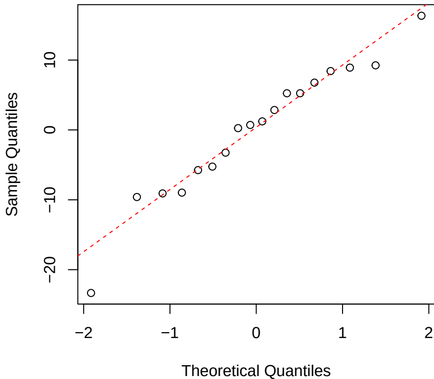
Cmass | 3000 | Weinmannia Normal Q-Q
