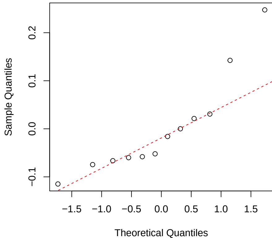
Toughness | 1000 | Clarisia Normal Q-Q
