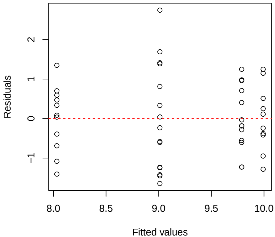
Nmass | 2000 | Myrcia Residuals vs Fitted
