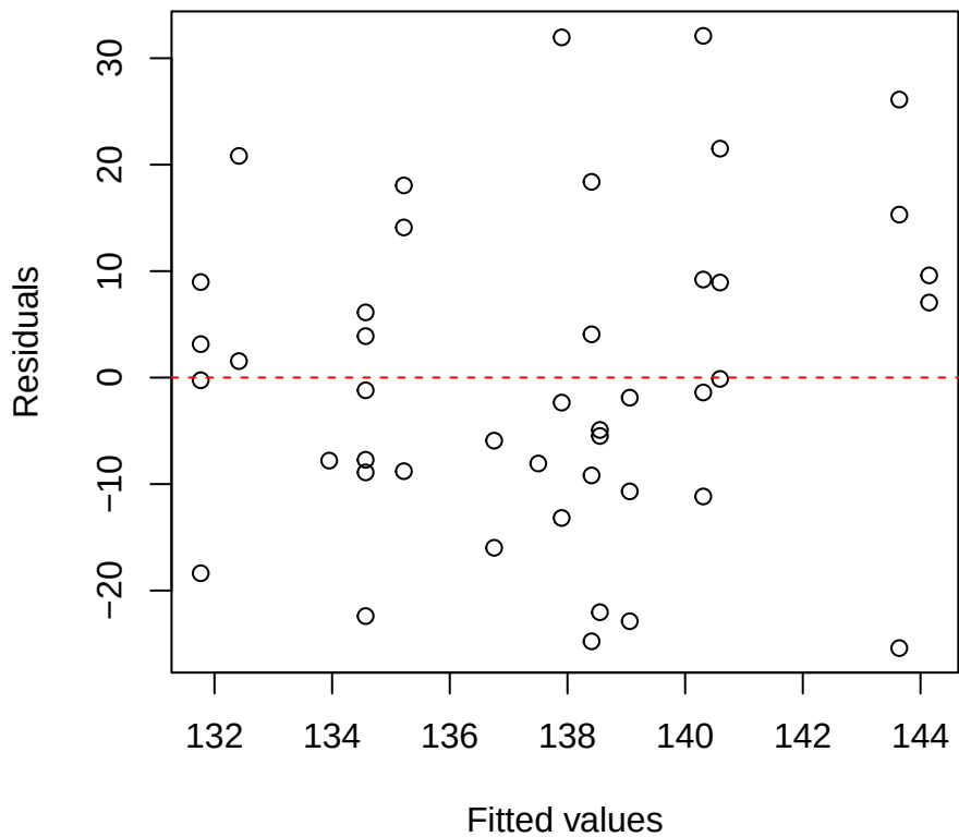
Carea | 2000 | Alchornea Residuals vs Fitted
