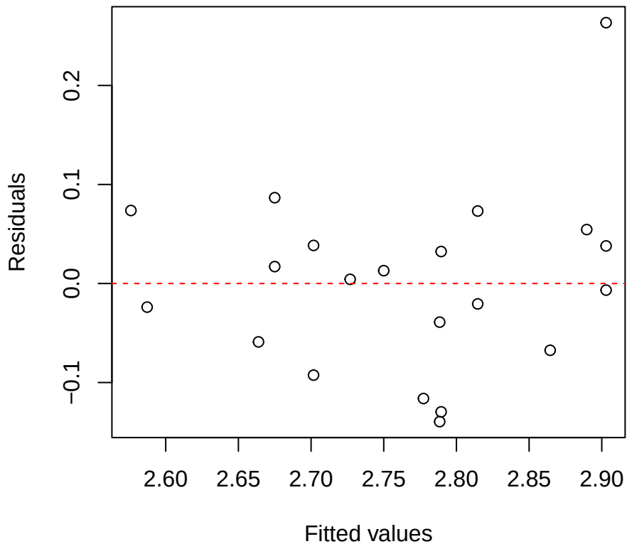
logNmass | 3000 | Hedyosmum Residuals vs Fitted
