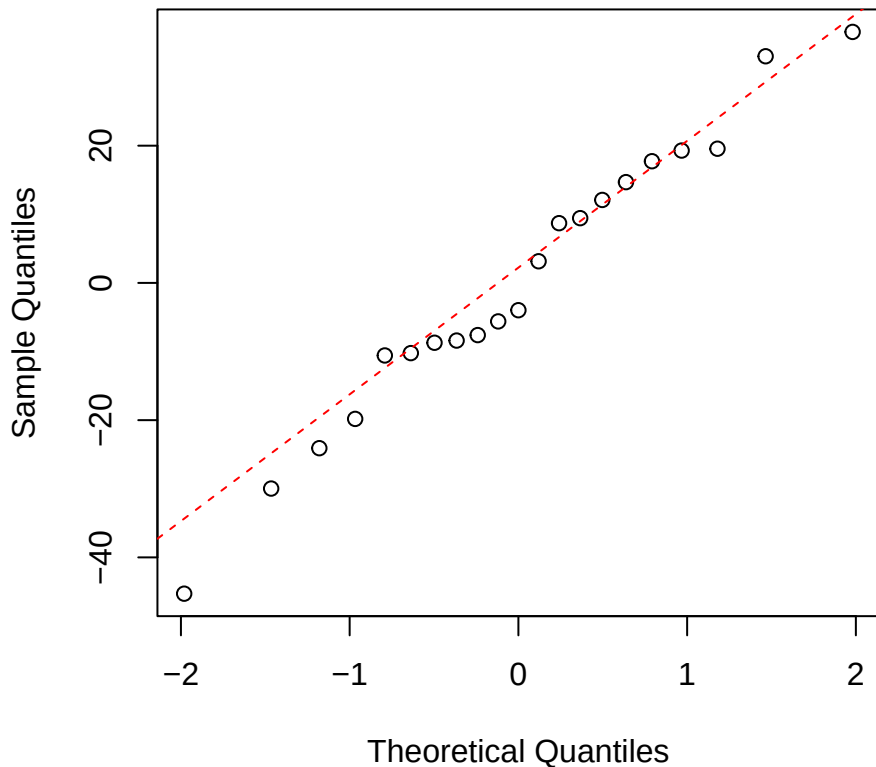
iWUE | 3000 | Hedyosmum Normal Q-Q
