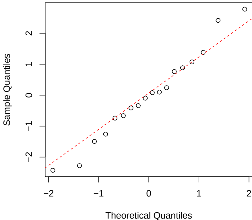
Nmass | 3000 | Weinmannia Normal Q-Q
