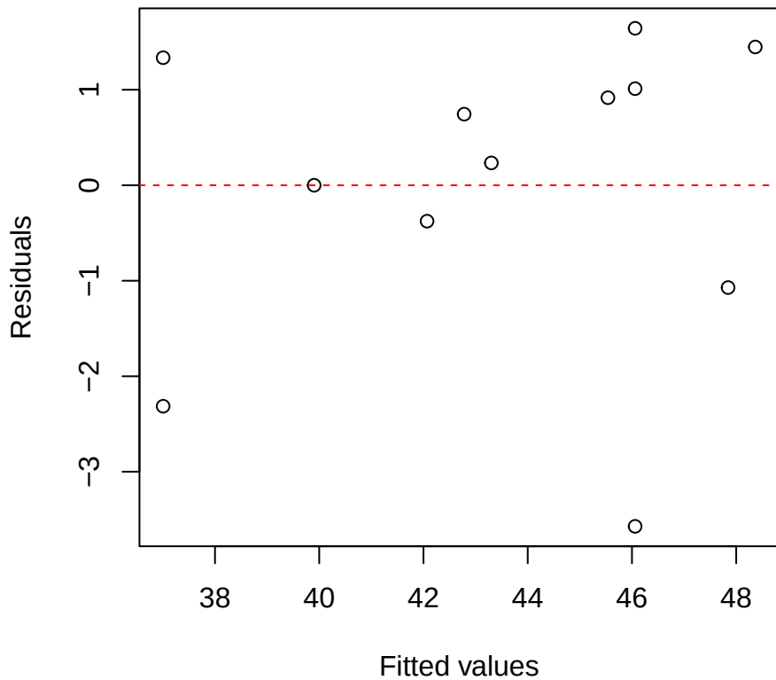
Carea | 1000 | Clarisia Residuals vs Fitted
