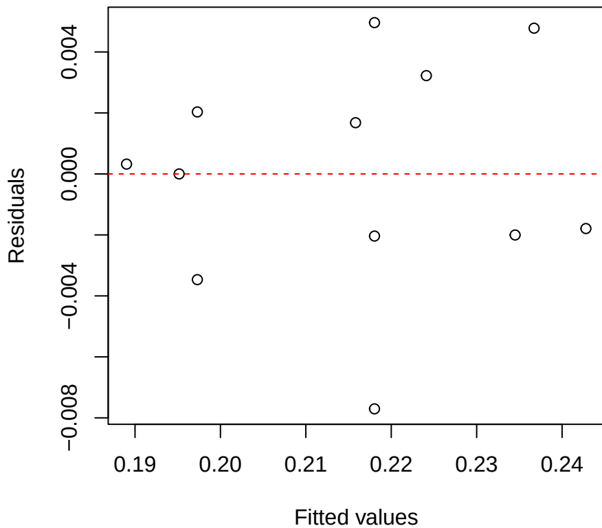
Thickness | 1000 | Clarisia Residuals vs Fitted
