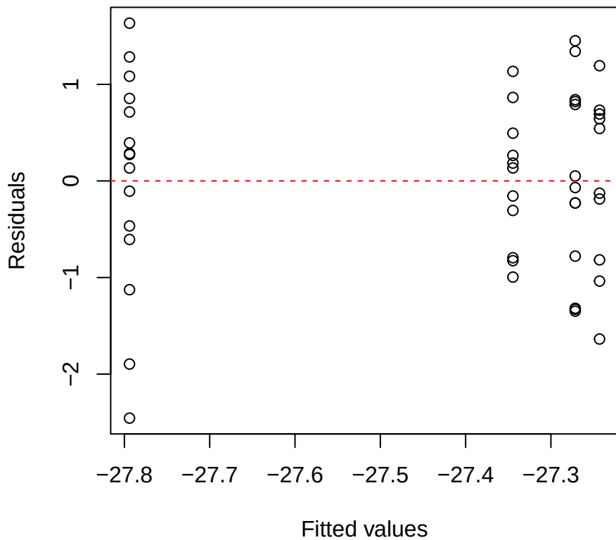
d13C | 2000 | Myrcia Residuals vs Fitted
