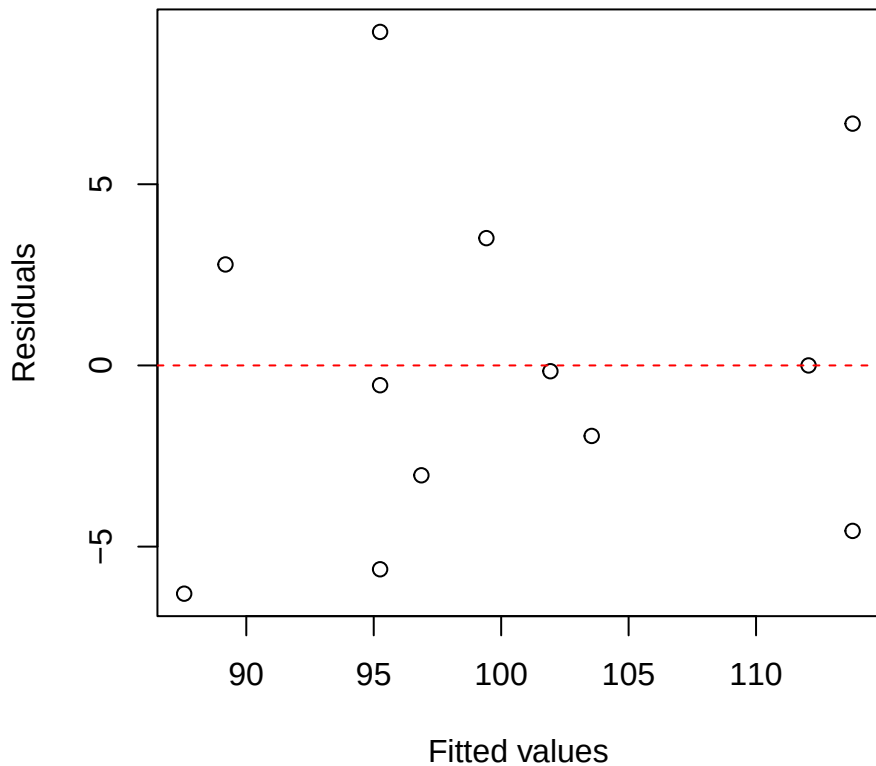
SLA | 1000 | Clarisia Residuals vs Fitted
