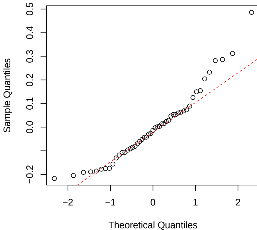
Toughness | 2000 | Myrcia Normal Q-Q
