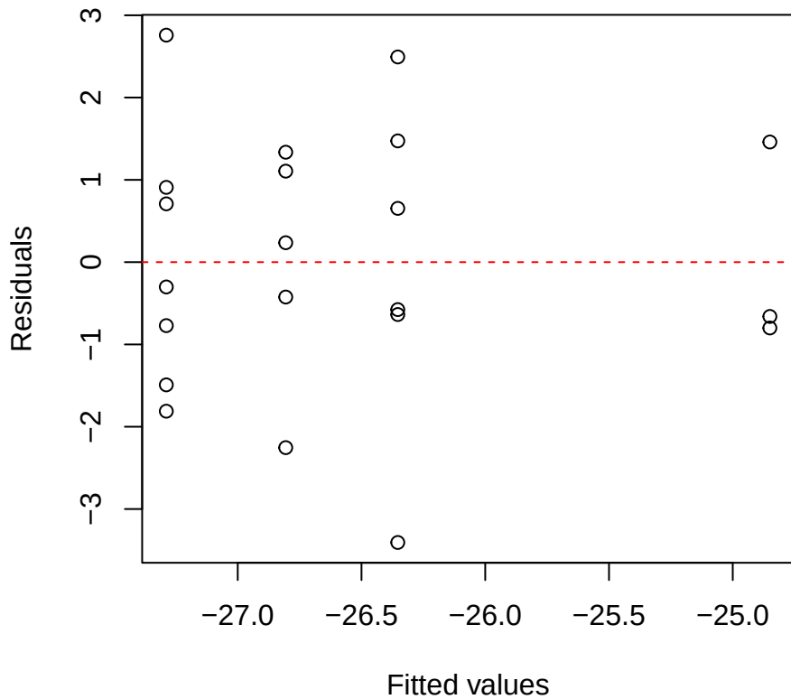
d13C | 3000 | Hedyosmum Residuals vs Fitted
