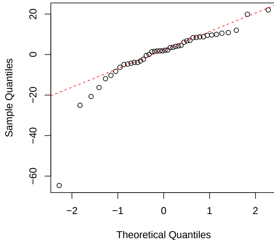
Cmass | 2000 | Alchornea Normal Q-Q
