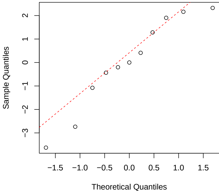
Nmass | 1000 | Clarisia Normal Q-Q
