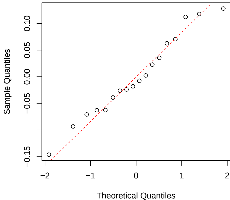
Toughness | 3000 | Weinmannia Normal Q-Q
