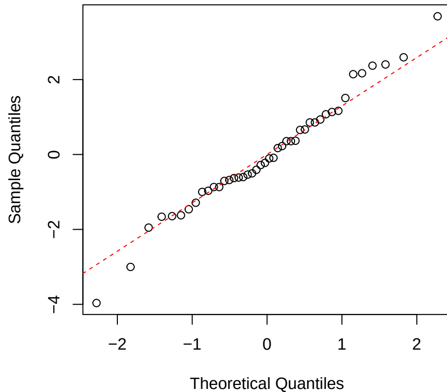
Nmass | 2000 | Alchornea Normal Q-Q
