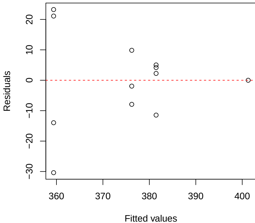
Ci | 1000 | Clarisia Residuals vs Fitted
