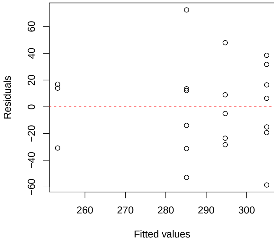
Ci | 3000 | Hedyosmum Residuals vs Fitted
