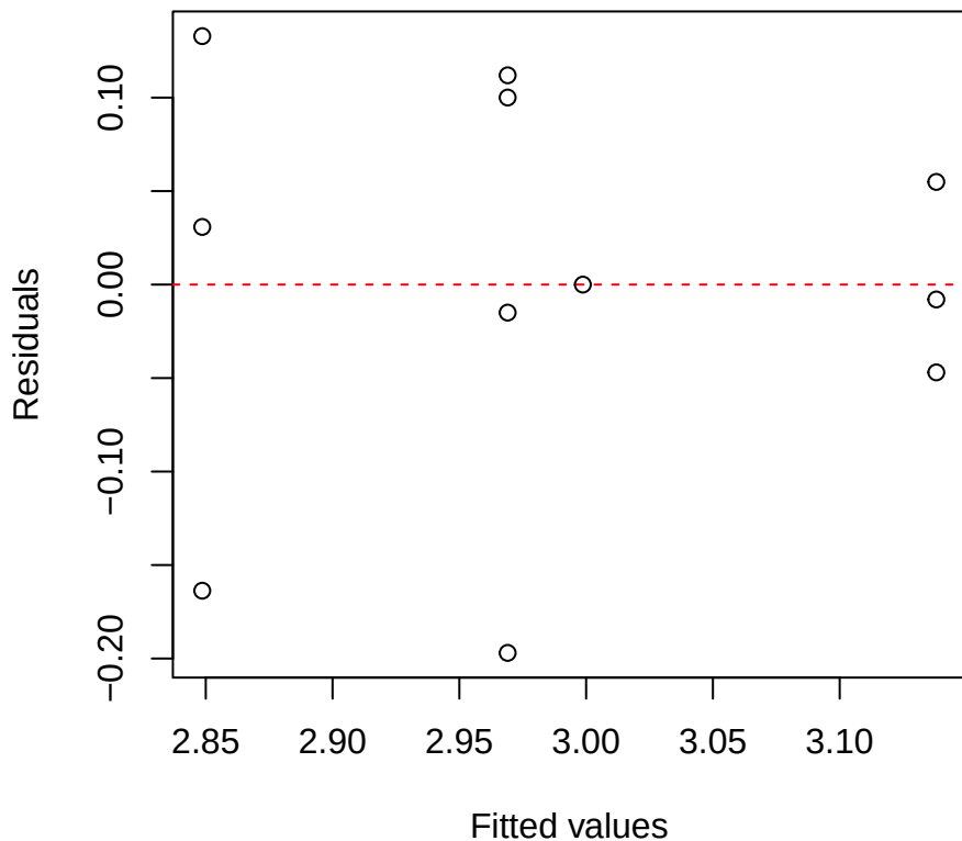
logNmass | 1000 | Clarisia Residuals vs Fitted
