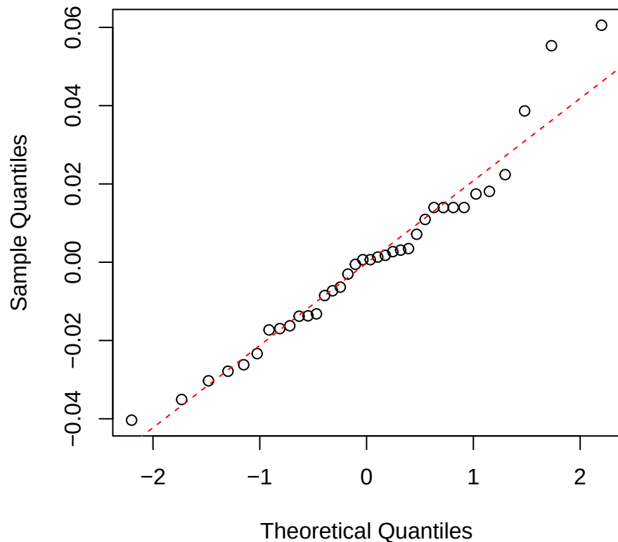
Thickness | 1000 | Pouteria Normal Q-Q
