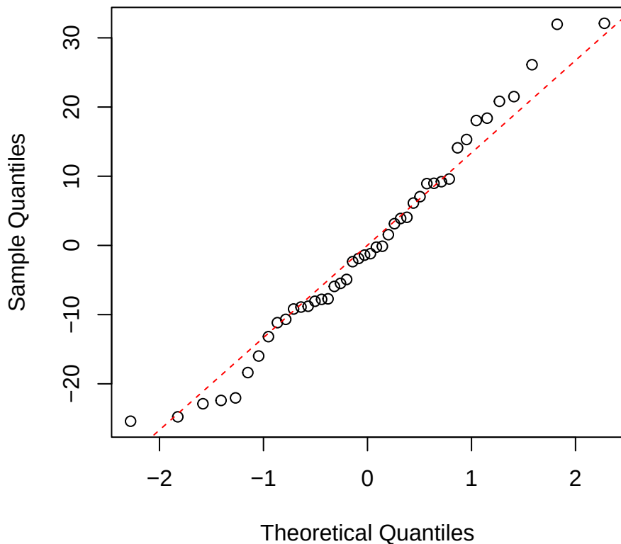
Carea | 2000 | Alchornea Normal Q-Q
