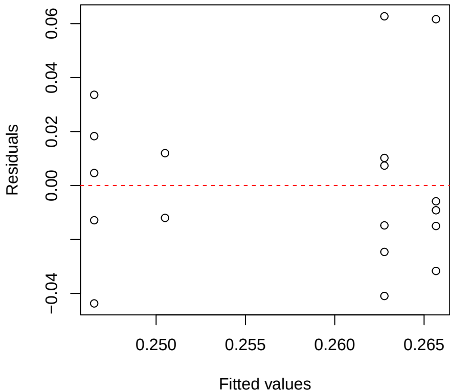
Thickness | 3000 | Weinmannia Residuals vs Fitted
