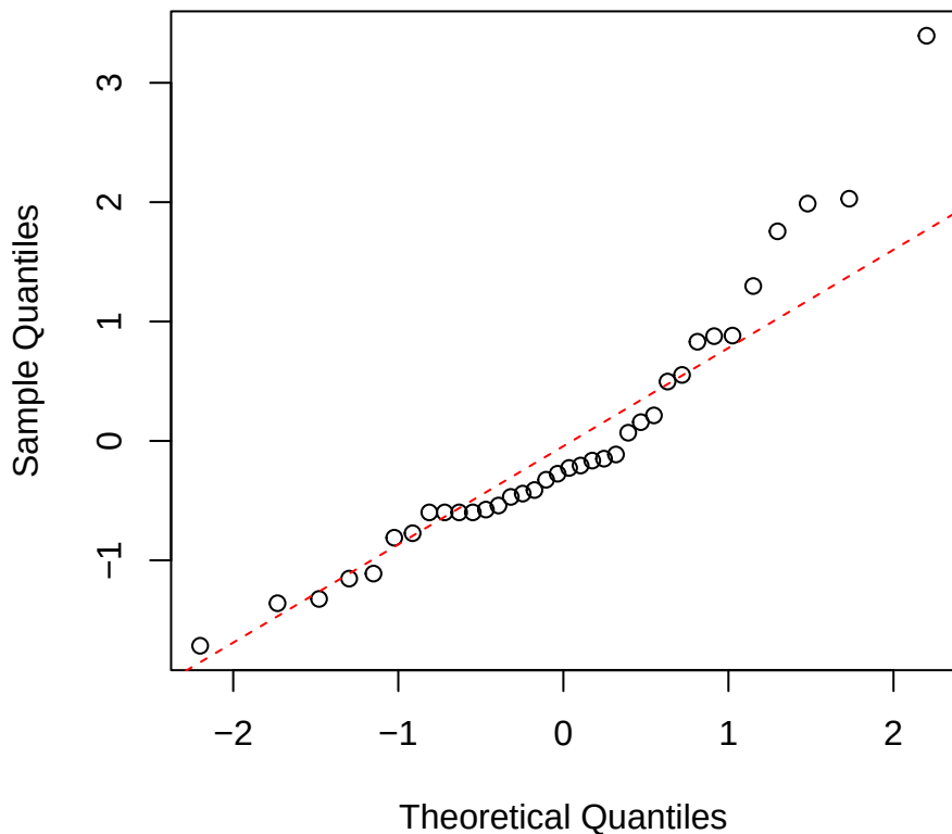
Nmass | 1000 | Pouteria Normal Q-Q
