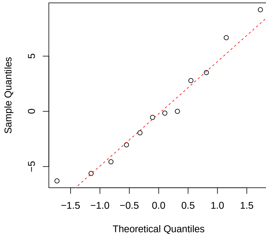
SLA | 1000 | Clarisia Normal Q-Q
