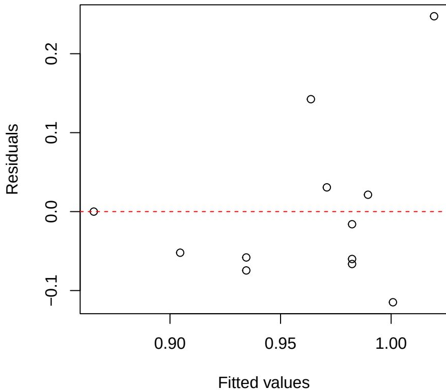
Toughness | 1000 | Clarisia Residuals vs Fitted
