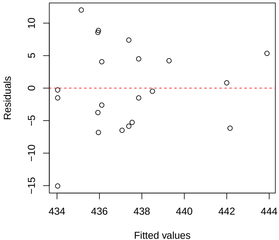
Cmass | 3000 | Hedyosmum Residuals vs Fitted
