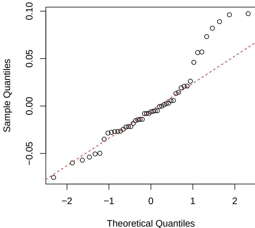
Thickness | 2000 | Myrcia Normal Q-Q
