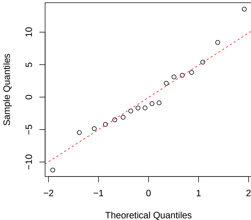
Carea | 3000 | Weinmannia Normal Q-Q
