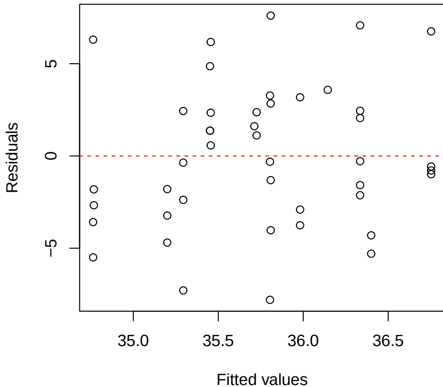
SLA | 2000 | Alchornea Residuals vs Fitted
