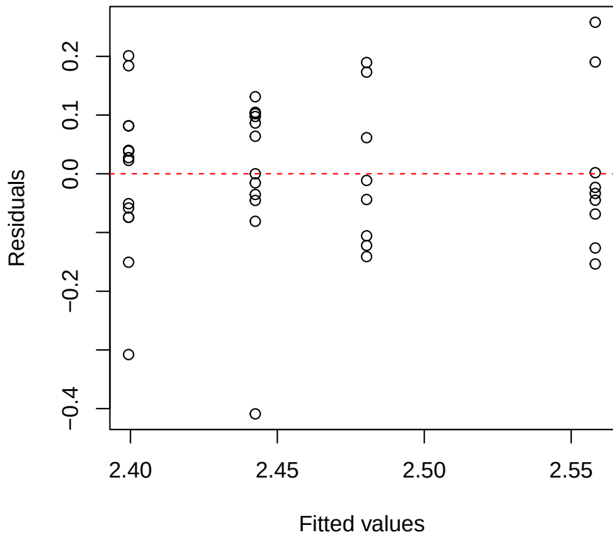
logNmass | 2000 | Alchornea Residuals vs Fitted
