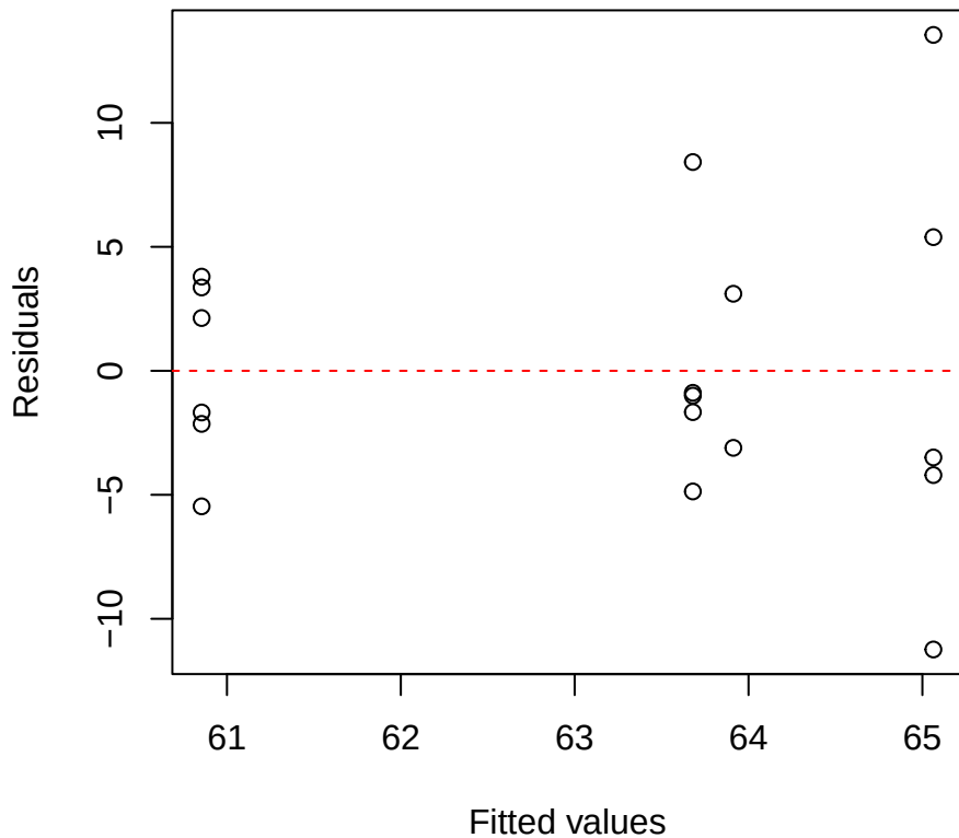
Carea | 3000 | Weinmannia Residuals vs Fitted
