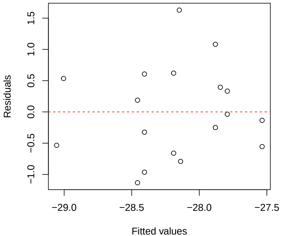
d13C | 3000 | Weinmannia Residuals vs Fitted
