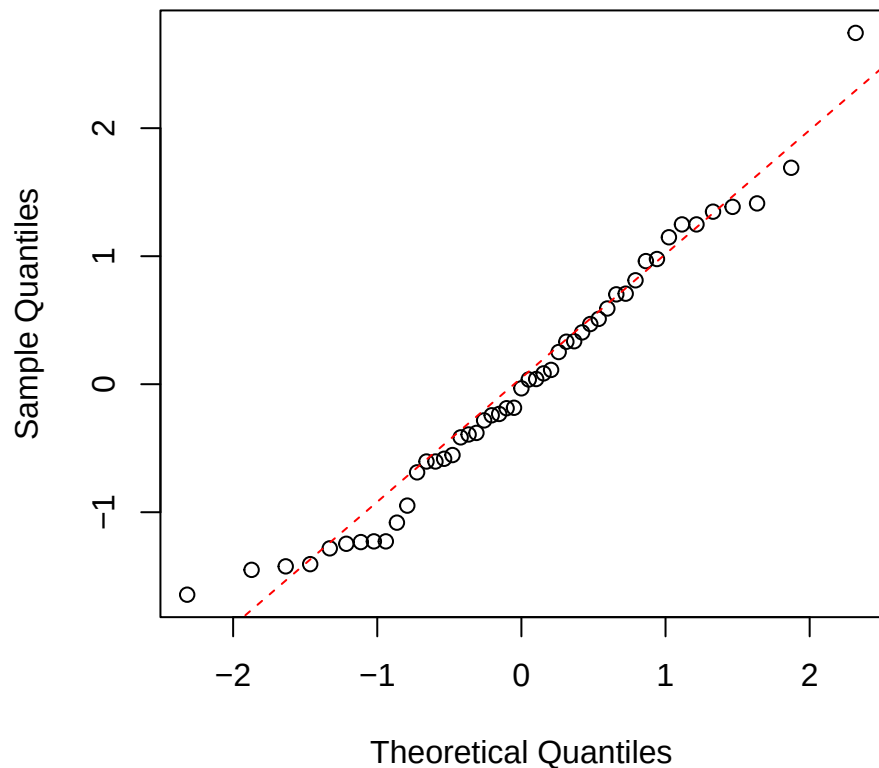
Nmass | 2000 | Myrcia Normal Q-Q
