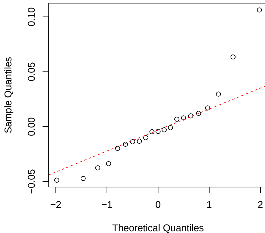
Thickness | 3000 | Hedyosmum Normal Q-Q
