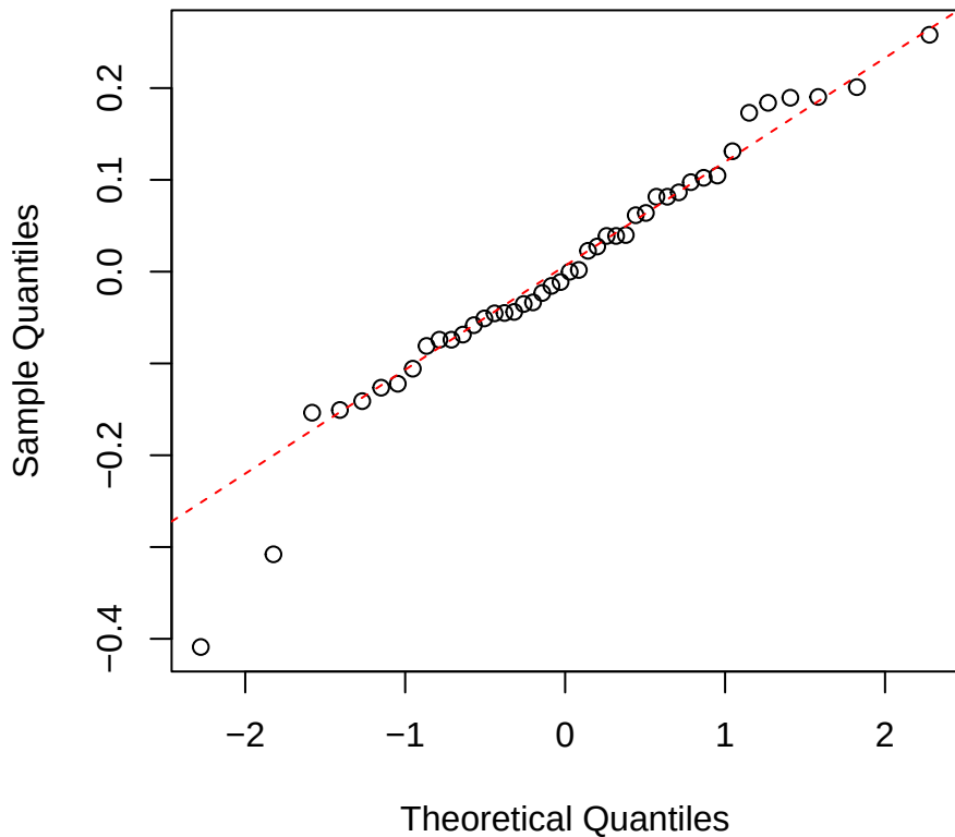
logNmass | 2000 | Alchornea Normal Q-Q
