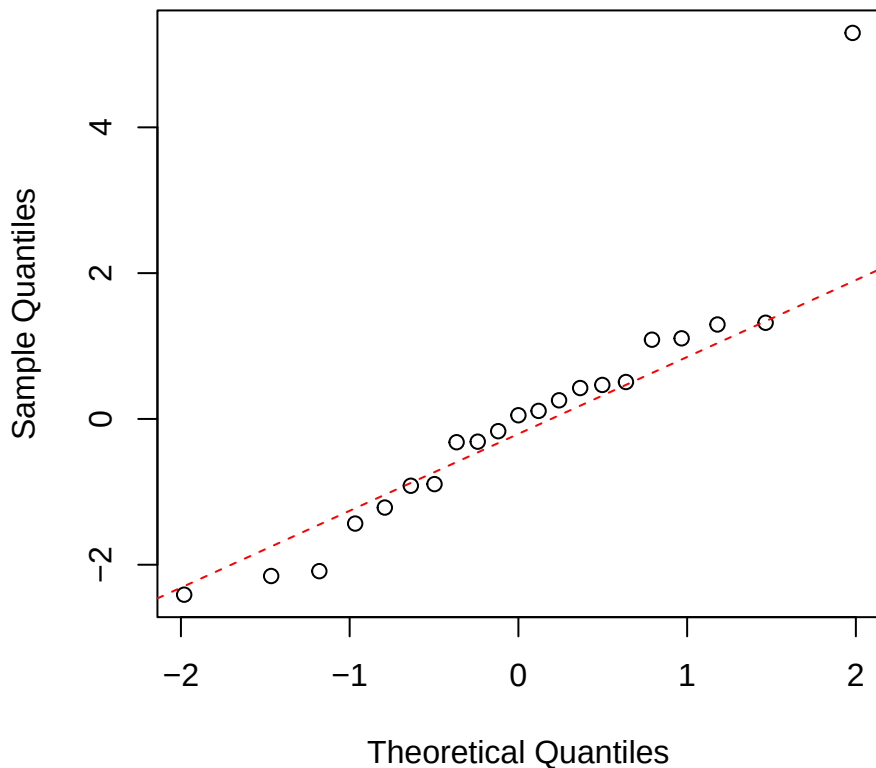
Nmass | 3000 | Hedyosmum Normal Q-Q
