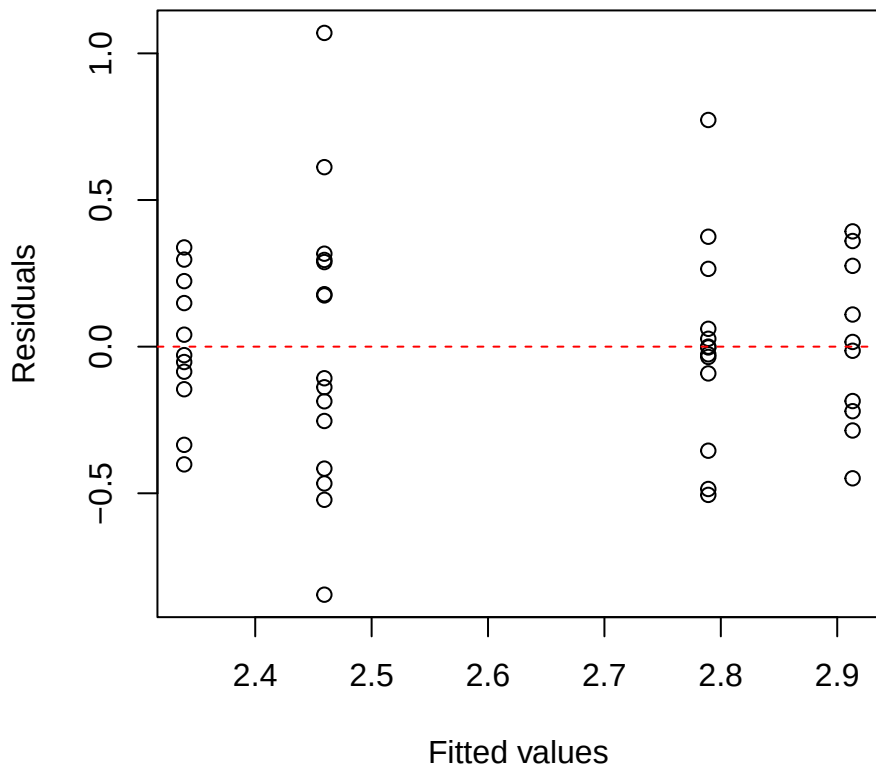
Narea | 2000 | Myrcia Residuals vs Fitted
