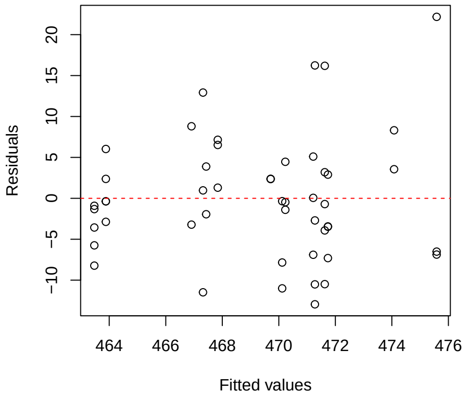
Cmass | 2000 | Myrcia Residuals vs Fitted
