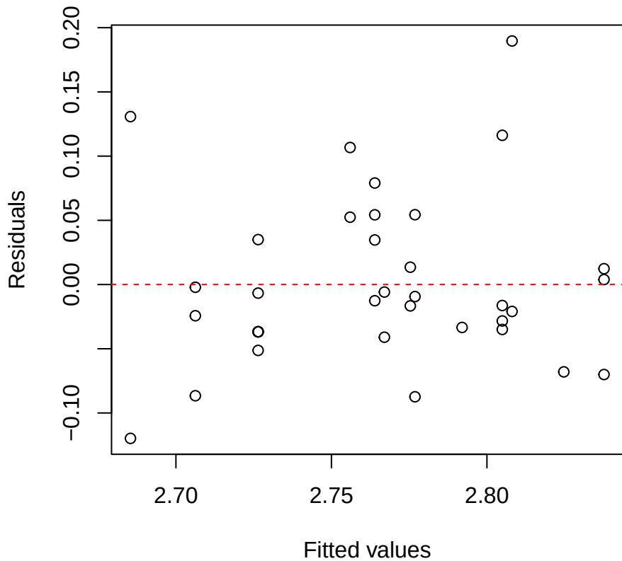
logNmass | 1000 | Pouteria Residuals vs Fitted
