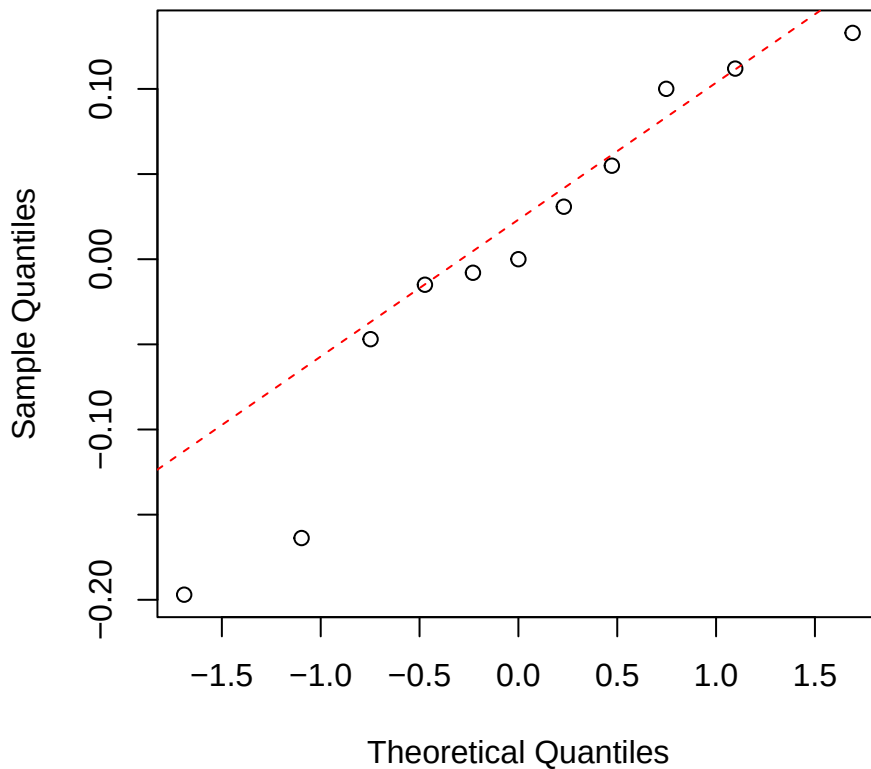
logNmass | 1000 | Clarisia Normal Q-Q
