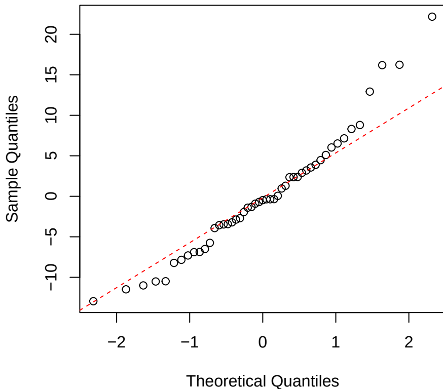
Cmass | 2000 | Myrcia Normal Q-Q
