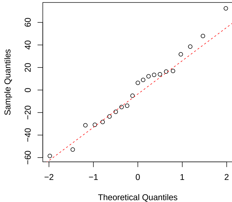
Ci | 3000 | Hedyosmum Normal Q-Q
