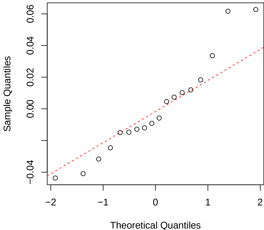
Thickness | 3000 | Weinmannia Normal Q-Q
