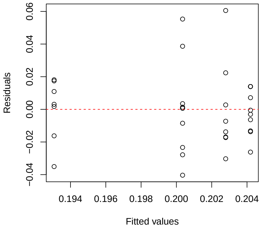
Thickness | 1000 | Pouteria Residuals vs Fitted
