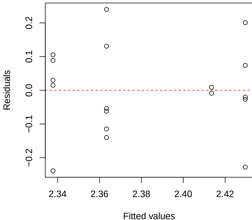
logNmass | 3000 | Weinmannia Residuals vs Fitted
