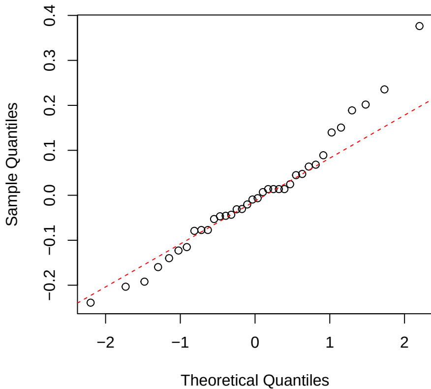
Toughness | 1000 | Pouteria Normal Q-Q
