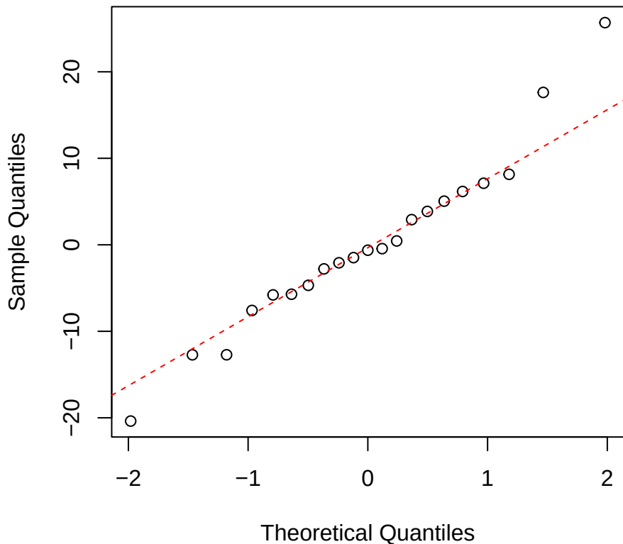
Carea | 3000 | Hedyosmum Normal Q-Q
