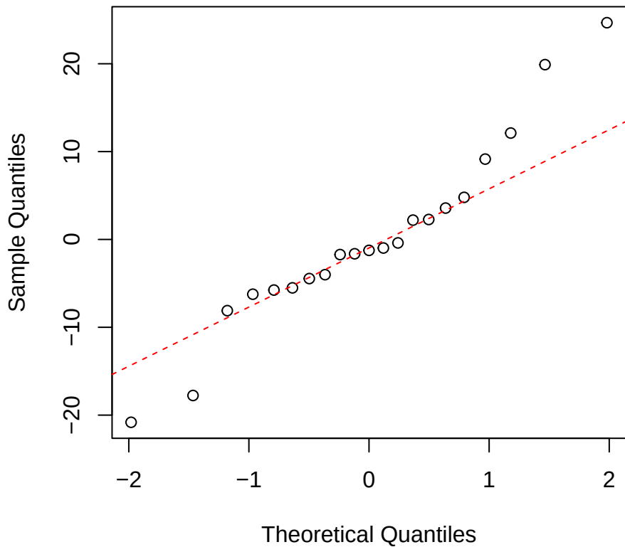
SLA | 3000 | Hedyosmum Normal Q-Q
