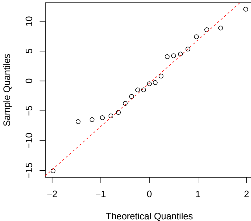
Cmass | 3000 | Hedyosmum Normal Q-Q
