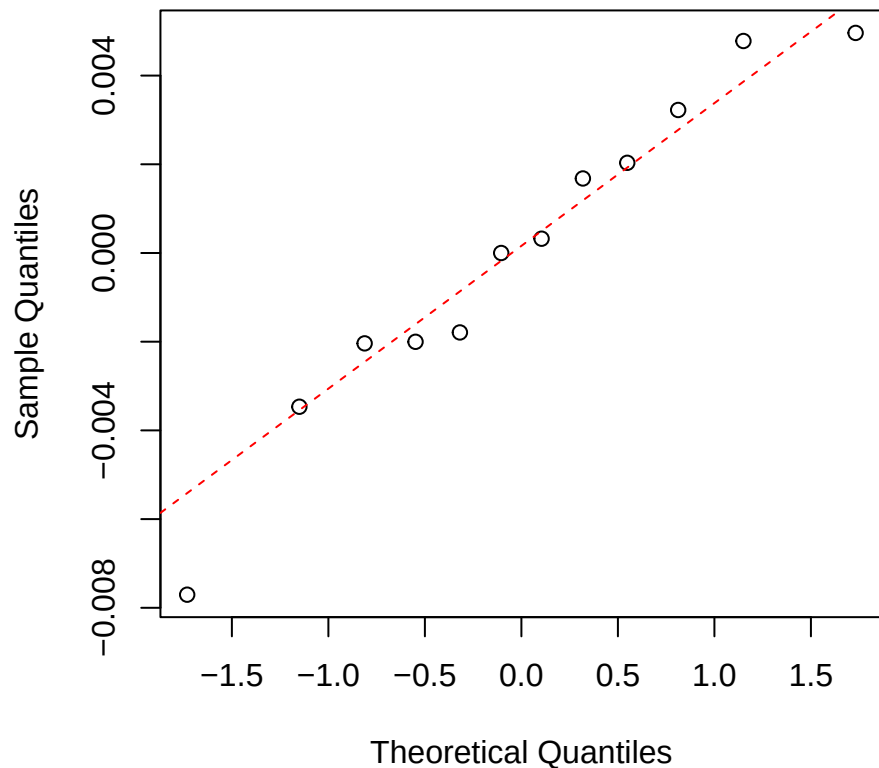
Thickness | 1000 | Clarisia Normal Q-Q
