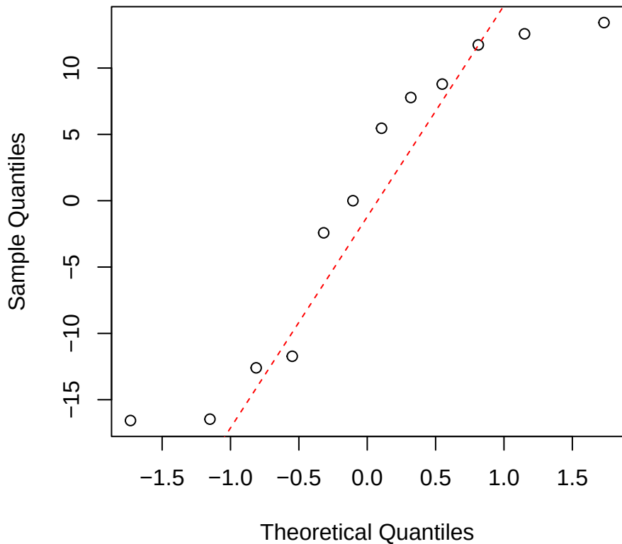
Cmass | 1000 | Clarisia Normal Q-Q
