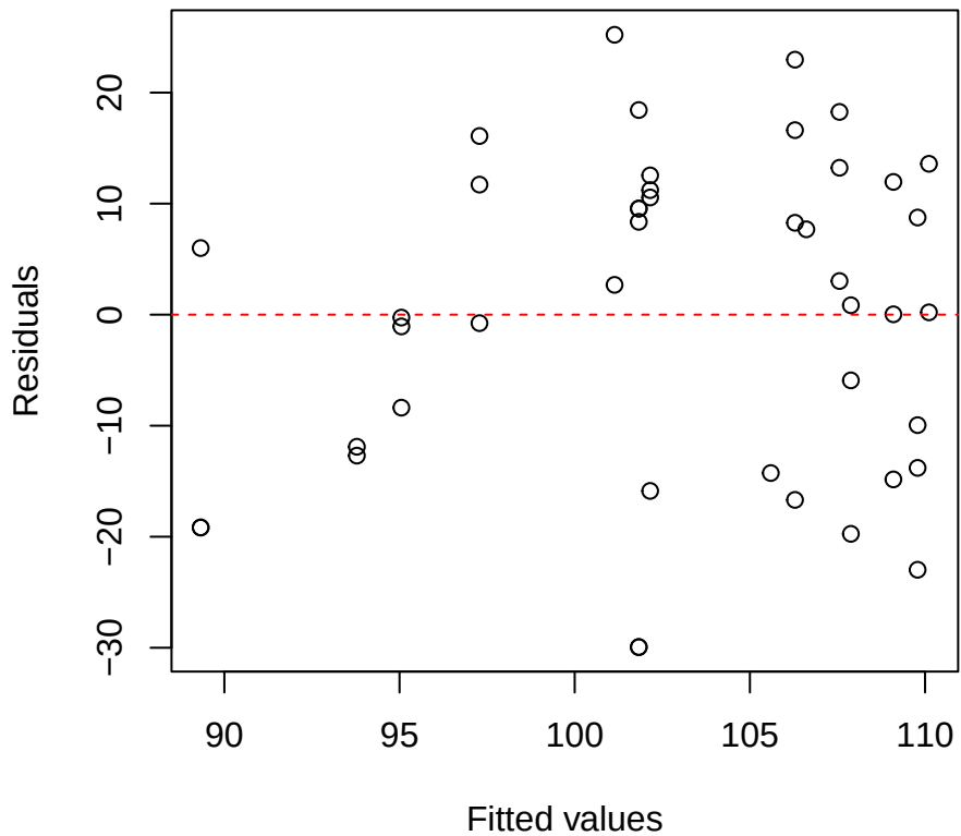
iWUE | 2000 | Alchornea Residuals vs Fitted
