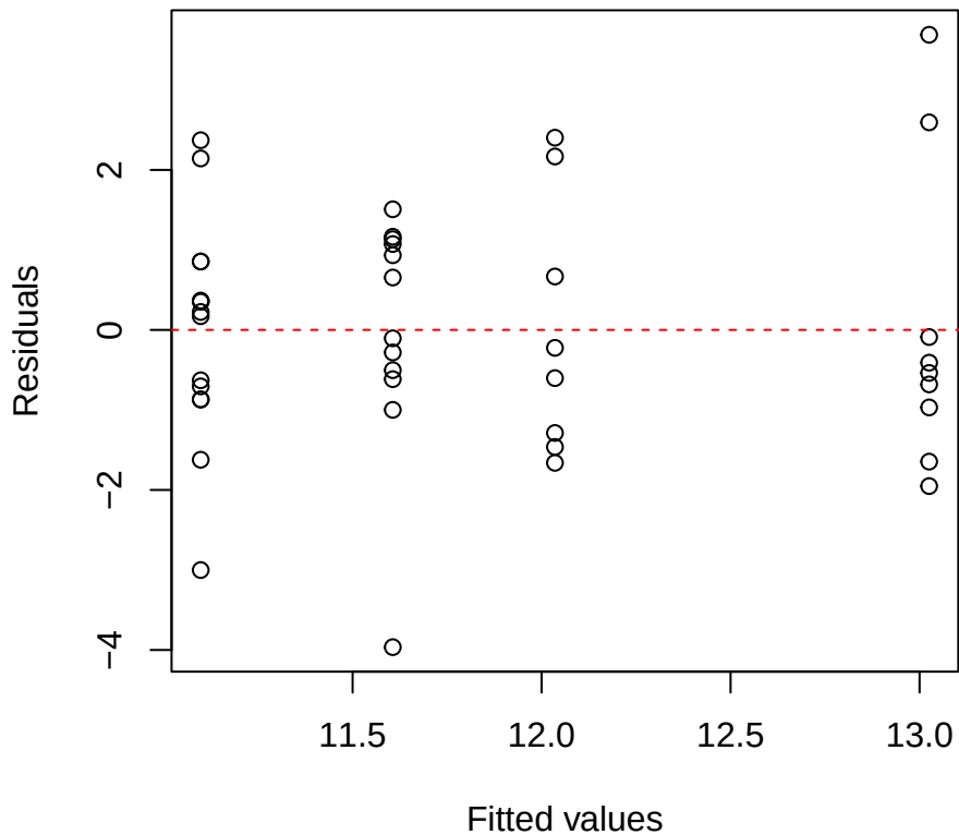
Nmass | 2000 | Alchornea Residuals vs Fitted
