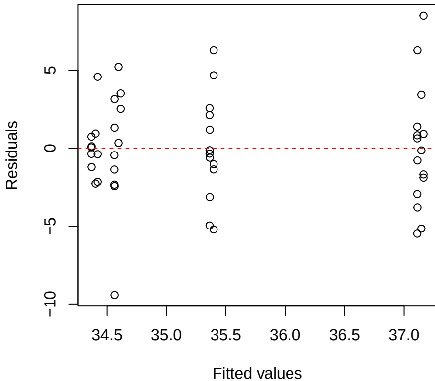
SLA | 2000 | Myrcia Residuals vs Fitted
