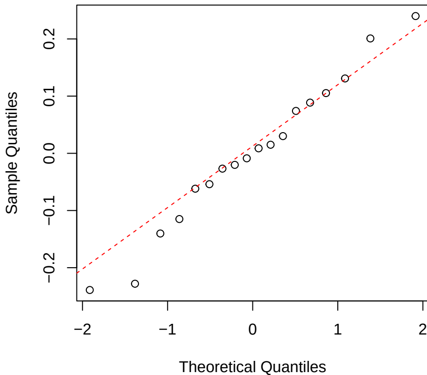
logNmass | 3000 | Weinmannia Normal Q-Q
