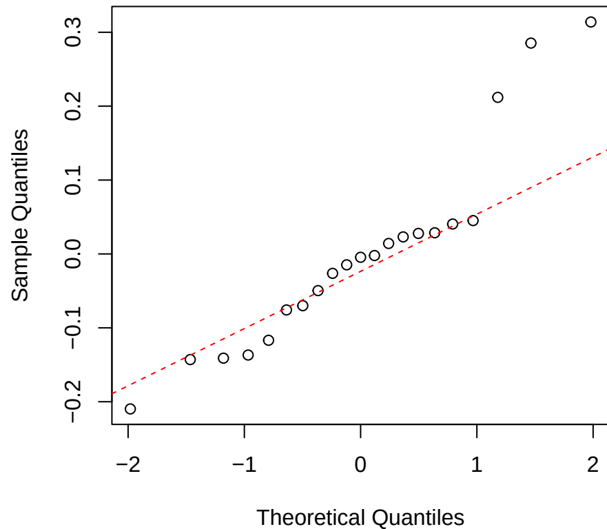
Toughness | 3000 | Hedyosmum Normal Q-Q
