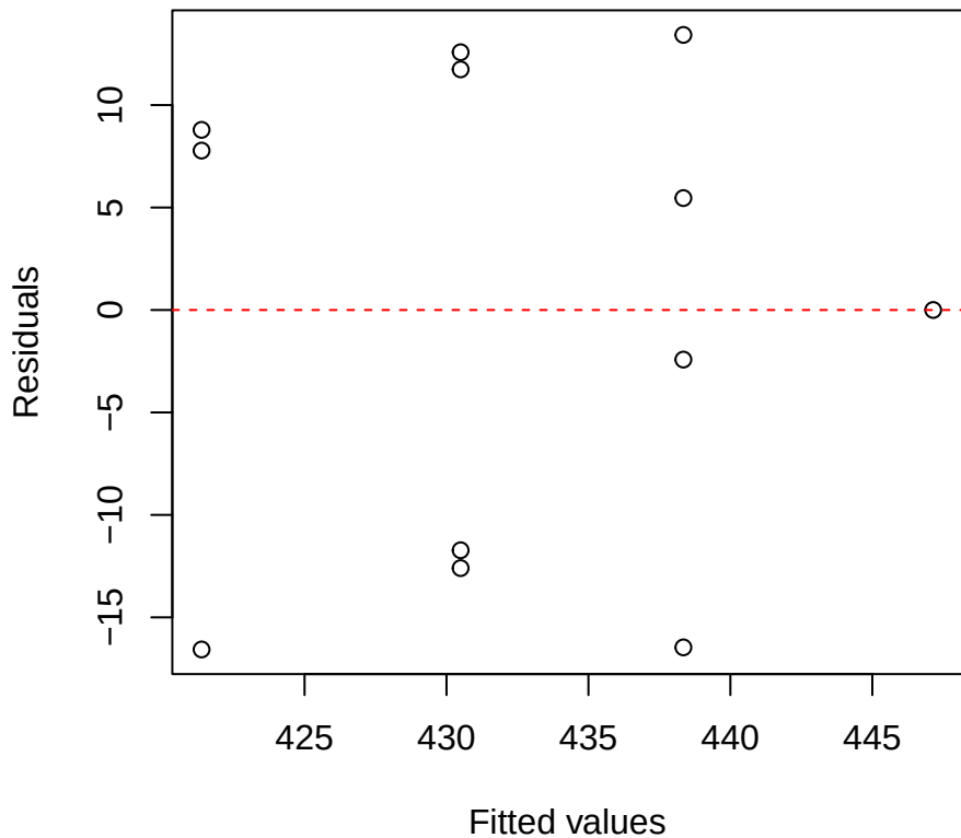
Cmass | 1000 | Clarisia Residuals vs Fitted
