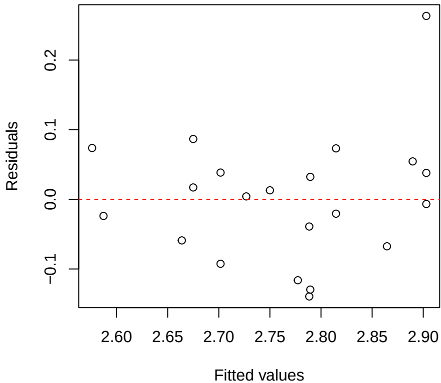
logNmass | 3000 | Hedyosmum Residuals vs Fitted
