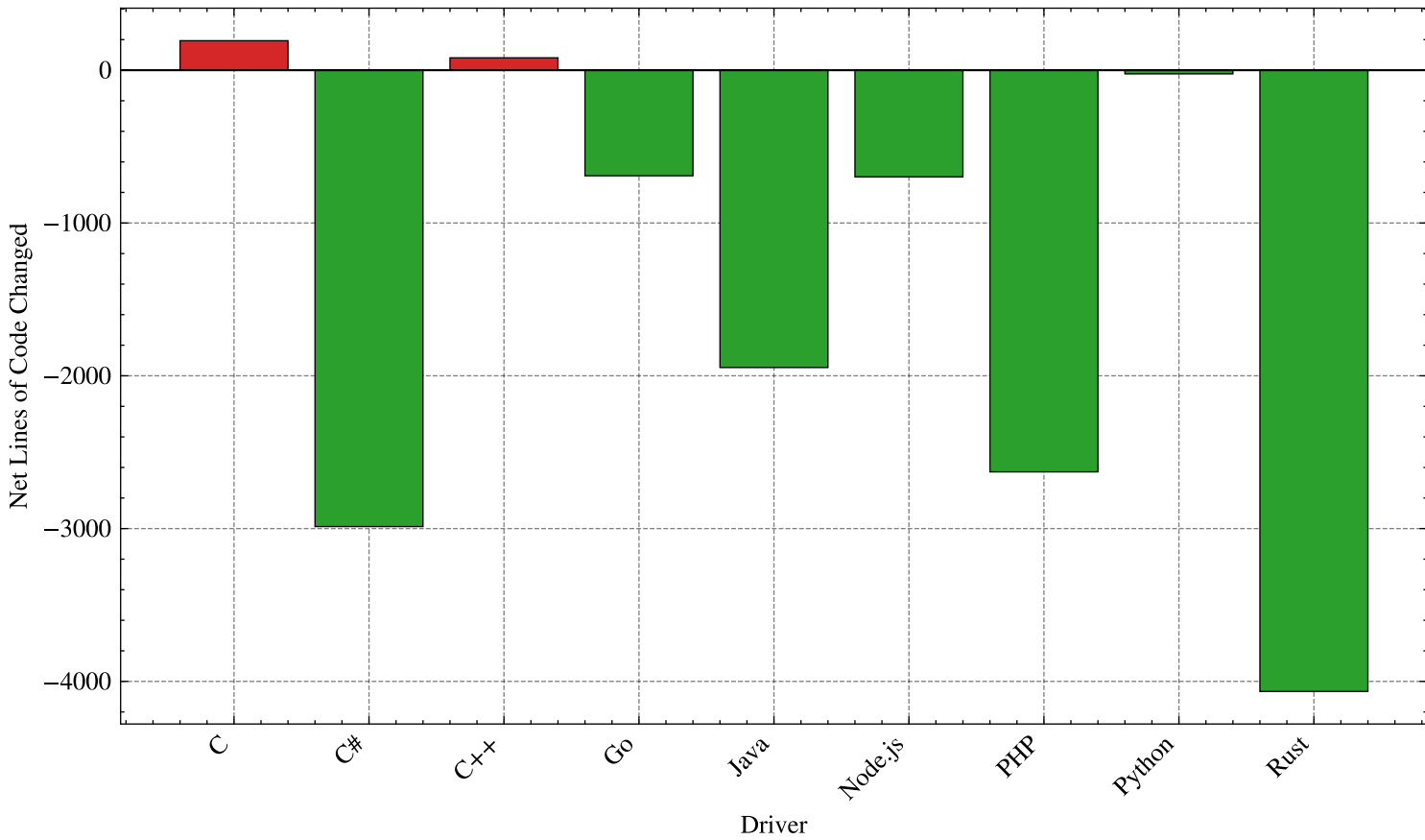
Unified Test Format Migration: Net Code Change by Driver
