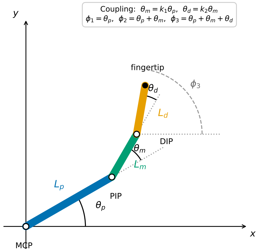
(A) Forward kinematics and the coupling constraint
