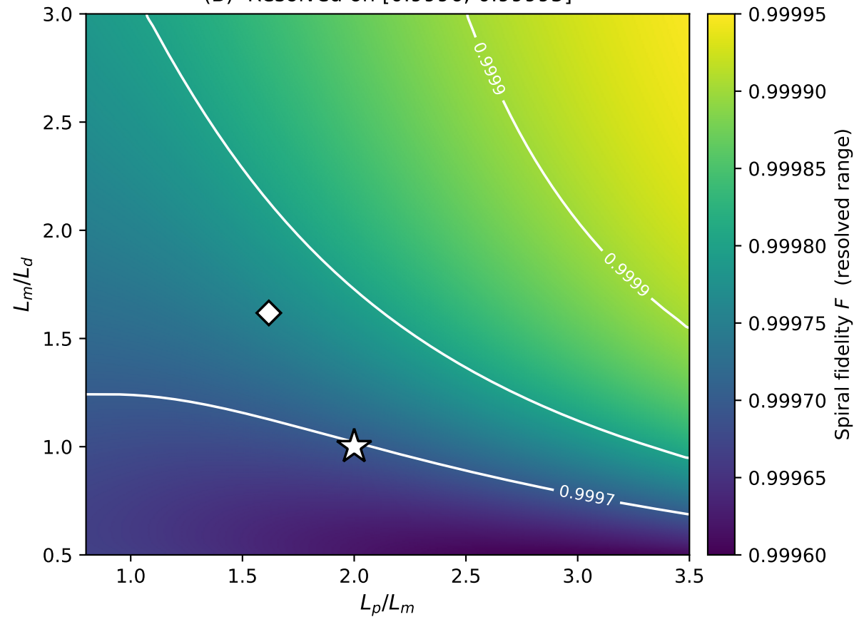
(B) Resolved on [0.9996, 0.99995]
