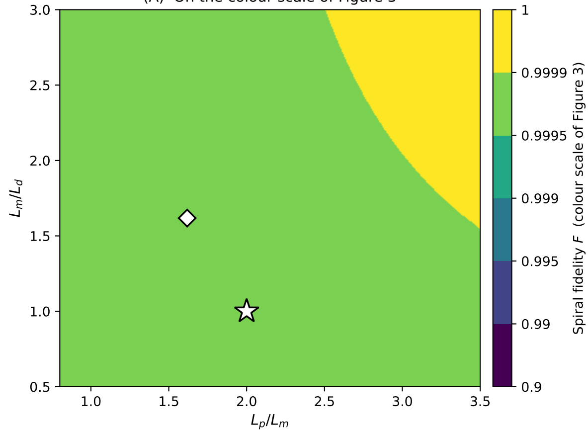
(A) On the colour scale of Figure 3
