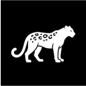
LEOPARD
