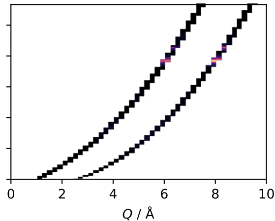
Kinematic constraints: TOSCA
