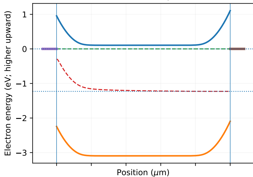
(a) Native STO facet junction
